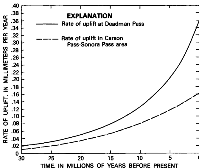
FIGURE 11.—Rate of uplift of crest of central Sierra Nevada at Deadman Pass and in Carson Pass-Sonora Pass area. Curves based on graphic differentiation of uplift curves in figure 10.
