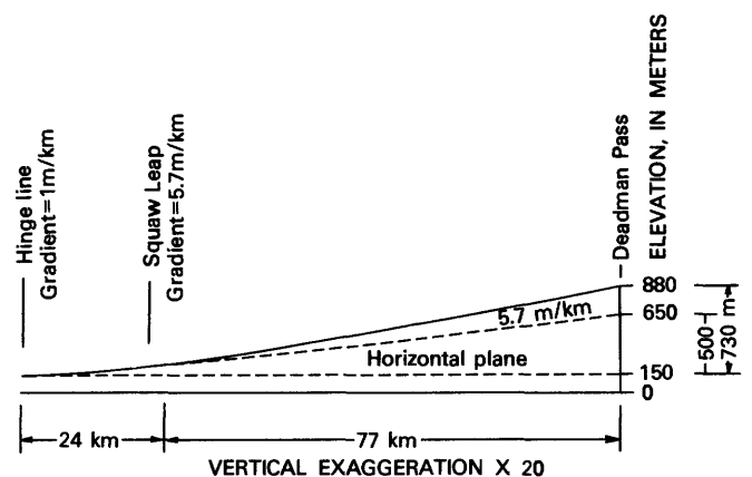
FIGURE 8.— Reconstruction of 10-m.y.-old profile of upper San Joaquin River projected to vertical plane striking N. 40° E. Elevation drop of 730 m between Deadman Pass and hinge line allows for increase in gradient east from Squaw Leap whereas 500-m drop does not.
