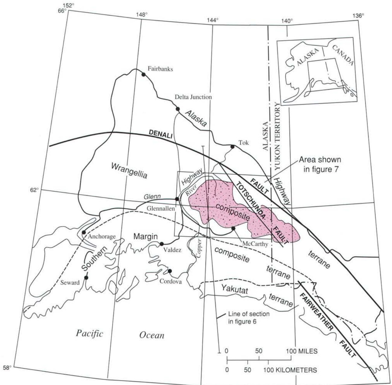
Figure 2. South-central Alaska and part of the Yukon Territory, Canada, showing Wrangell volcanic field (red stippled) and some major geologic features. Lines of faults dotted where concealed by water; dashed lines, terrane boundaries, where not depicted as faults.
