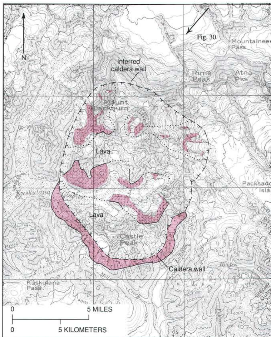
Figure 29. Topographic and generalized geologic map of Mount Blackburn. All remaining Mount Blackburn lavas are confined to an inferred caldera whose walls are mostly ice covered. Red stippled areas, granitic rocks of a postulated exhumed magma chamber in caldera; red crossed area, older syncaldera granites. Arrow indicates direction of view in figure 30. Base from U.S. Geological Survey McCarthy quadrangle map.
