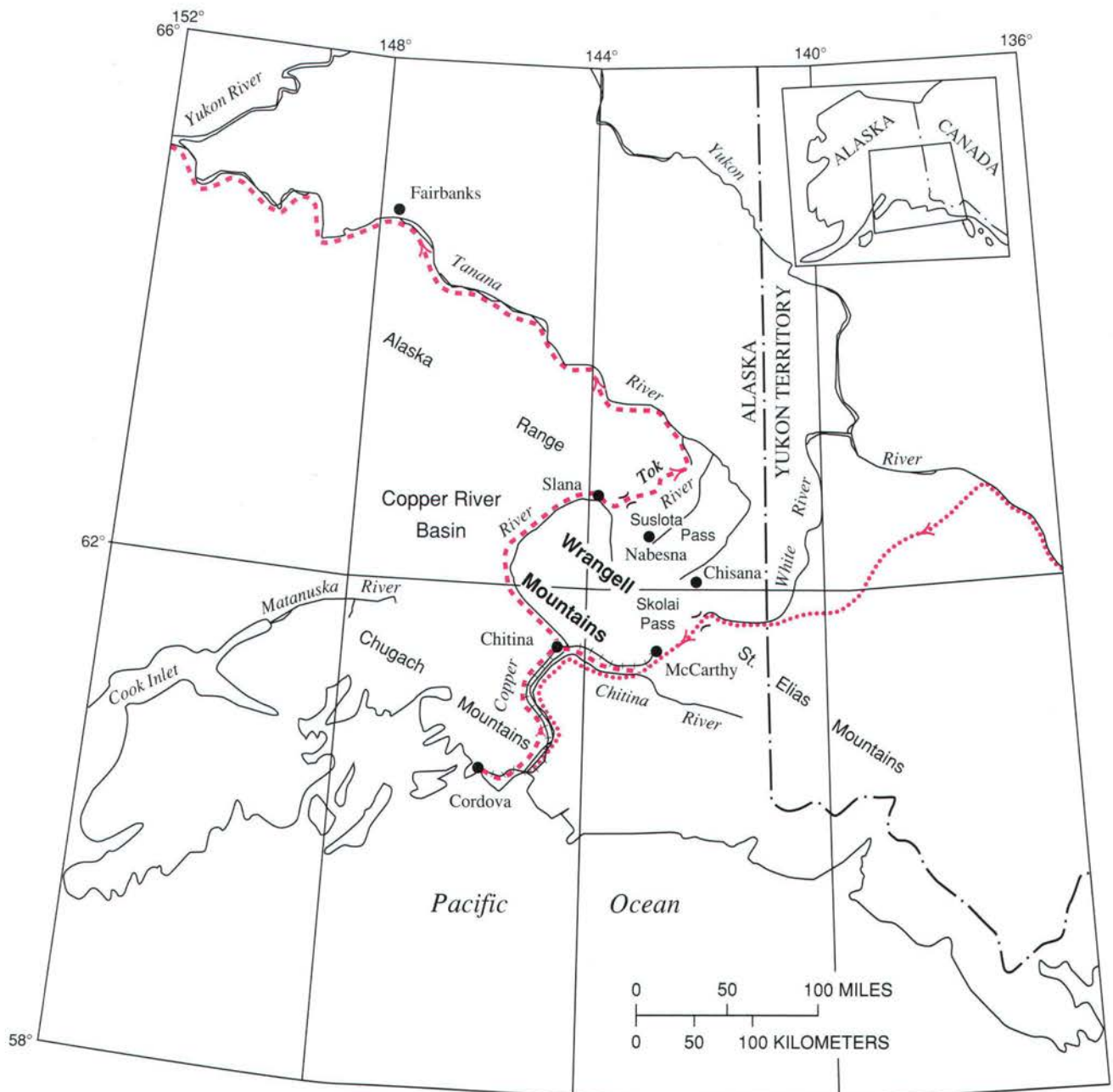
Figure 1. South-central Alaska and part of the Yukon Territory, Canada, showing early exploration routes of Allen in 1885 (red dashed line) and Schwatka and Hayes in 1891 (red dotted line) and route of the Cordova-Kennicott Railroad (barred line) that was used from 1911 to 1938.
