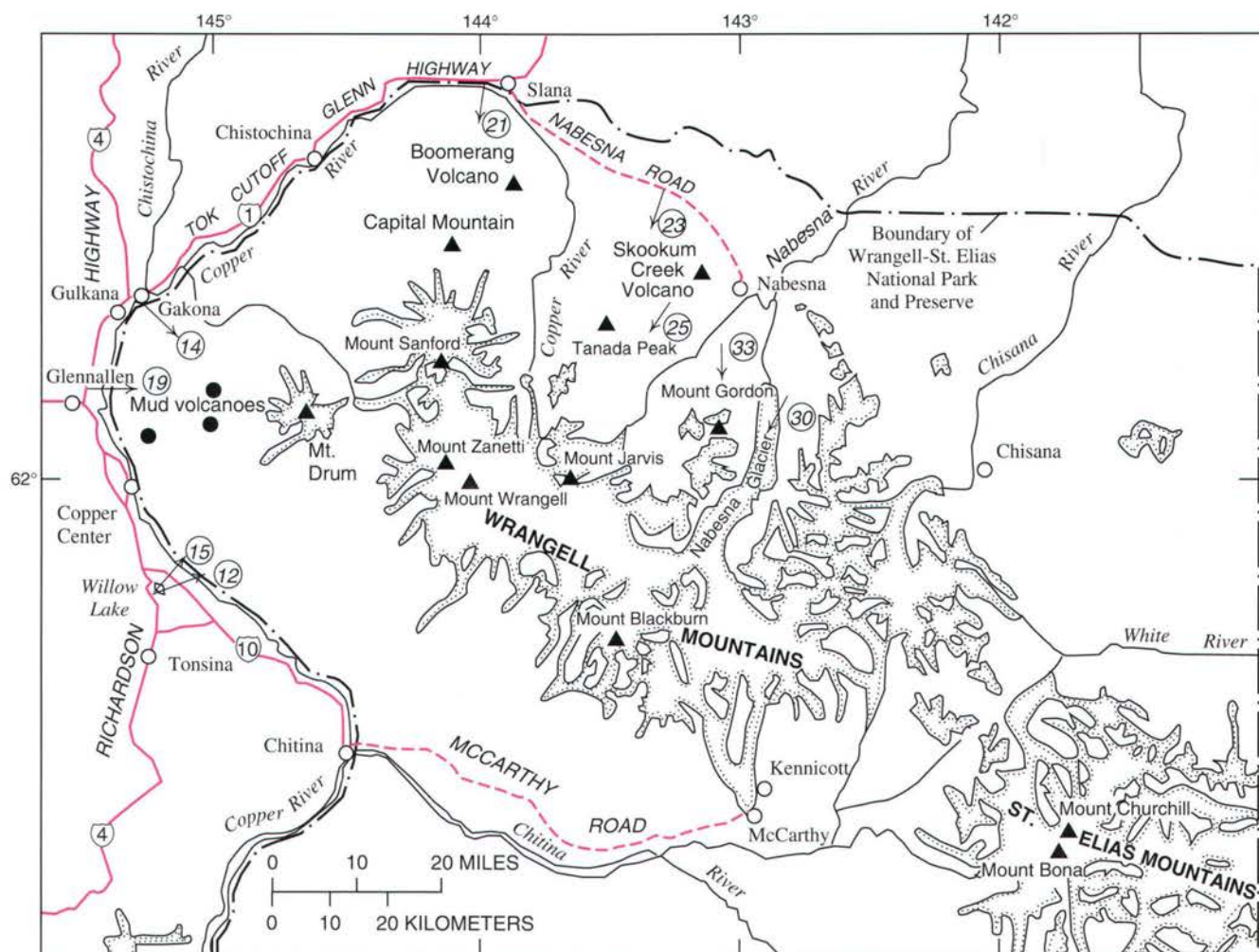
Wrangell Mountains and part of the St. Elias Mountains, showing locations of volcanoes and other geologic features discussed in text. Stippled lines, areas of icefields and glaciers. Arrows indicate accessible viewing areas discussed in text; circled numbers refer to figures showing photographs of volcanoes.
