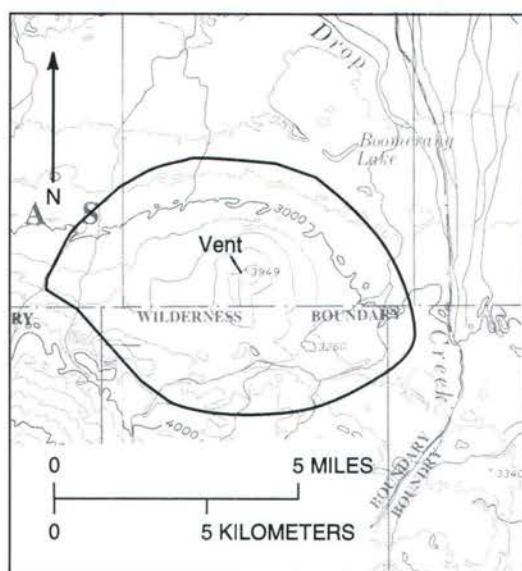
Figure 31. Topographic and generalized geologic map of Boomerang volcano. Heavy line, approximate present limit of Boomerang lavas. Peak at 3,949 ft is on small crater that was site of central-vent activity. Base from U.S. Geological Survey Nabesna quadrangle map.
