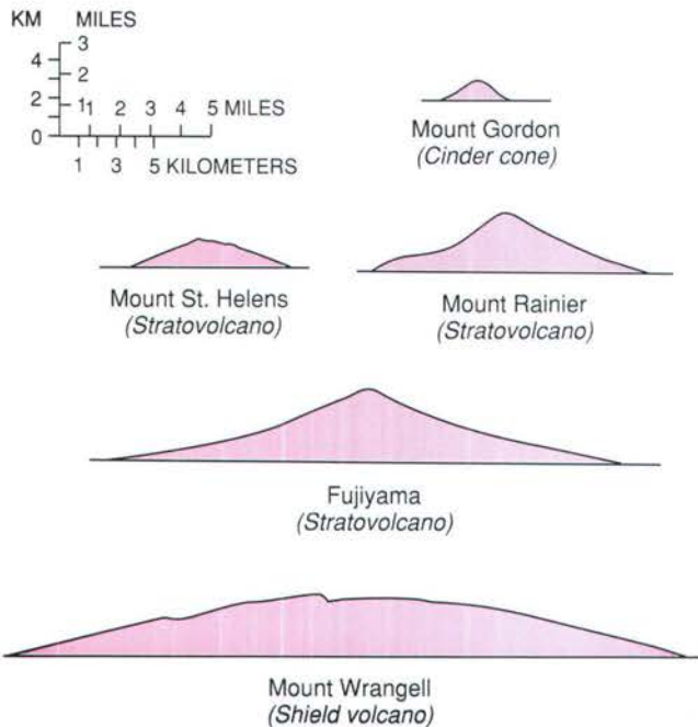
Figure 10. Comparative profiles of some Pacific-rim volcanoes. Mount Gordon, a cinder cone, and Mount Wrangell, a shield volcano, are described in text; Mount St. Helens, Mount Rainier, and Fujiyama are well-known stratovolcanoes.
