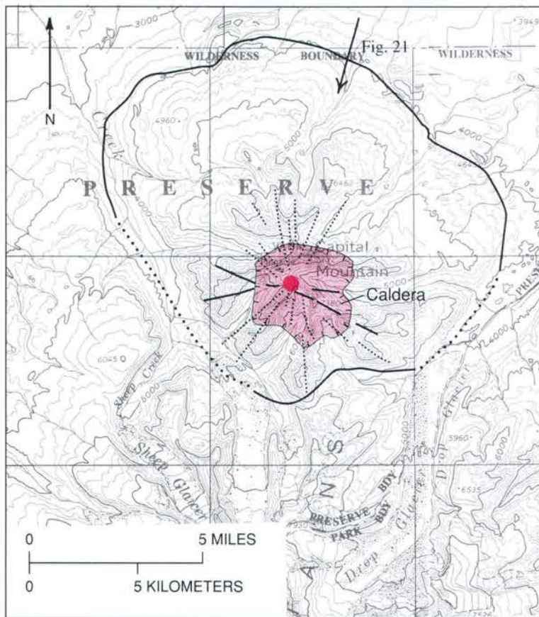
Figure 20. Topographic and generalized geologic map of Capital Mountain. Heavy line, approximate present limit of Capital Mountain lavas, dotted where concealed by young surficial deposits; dashed (rhyolite dike) and dotted (andesite dikes) lines, radial dike swarm; dot, intracaldera plug. Arrow indicates direction of view in figure 21. Base from U.S. Geological Survey Gulkana and Nabesna quadrangle maps.
