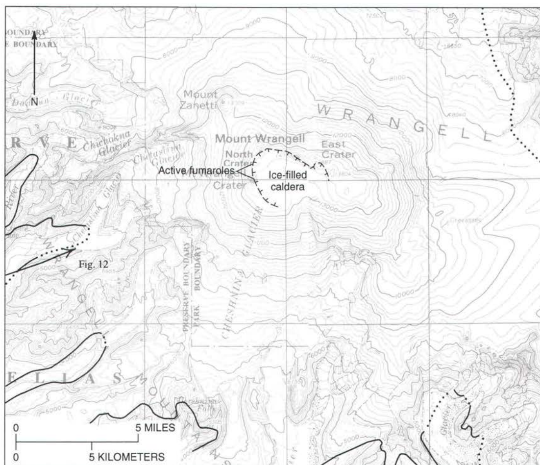
Figure 11. Topographic and generalized geologic map of Mount Wrangell. Heavy lines, approximate present limit of Mount Wrangell lavas, dotted where concealed by ice. Arrow indicates direction of view in figure 12. Base from U.S. Geological Survey Gulkana, Nabesna, Valdez, and McCarthy quadrangle maps.
