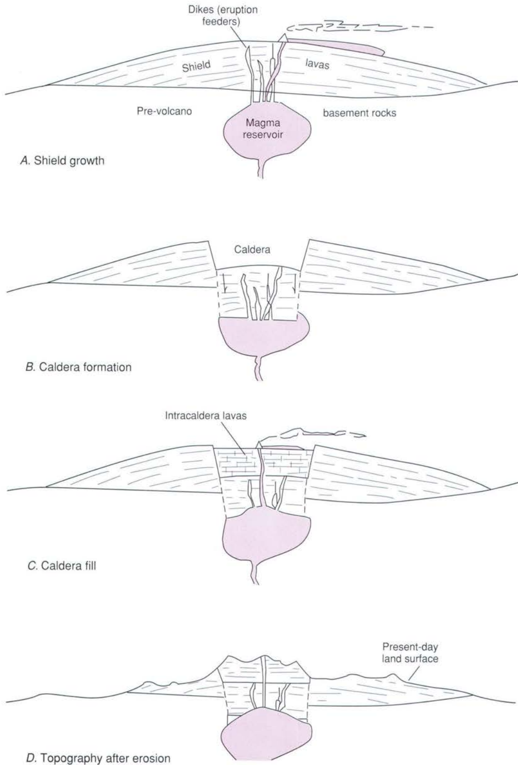
Figure 8. Diagrammatic cross section model illustrating development of a Wrangell volcano. A , Growth of shield by outpourings of voluminous lava flows from summit and rift vents. B , Collapse of summit caldera due to withdrawal of magma from a high-level magma reservoir. C , Filling of caldera by lava flows erupted from intracaldera vents. D , Present topography after erosion. Profile is that of Tanada volcano from mile 26 on the Nabesna Road. Growth of shield and collapse and filling of caldera probably occur partly concurrently.
