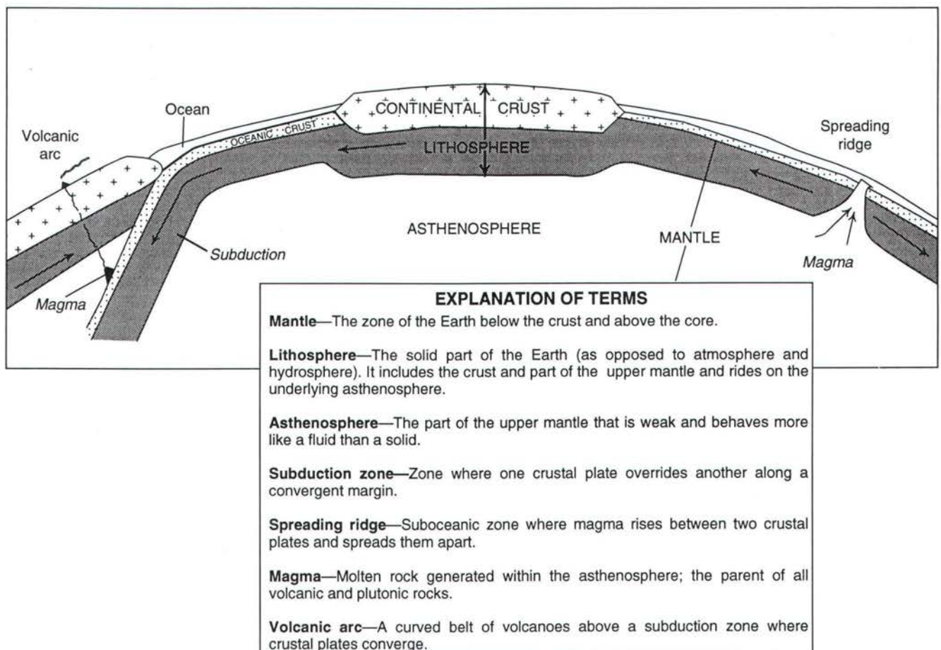
Figure 5. Diagrammatic cross section through the Earth's crust and upper mantle, showing plate-tectonic features discussed in text. Arrows indicate directions of relative plate motion.
