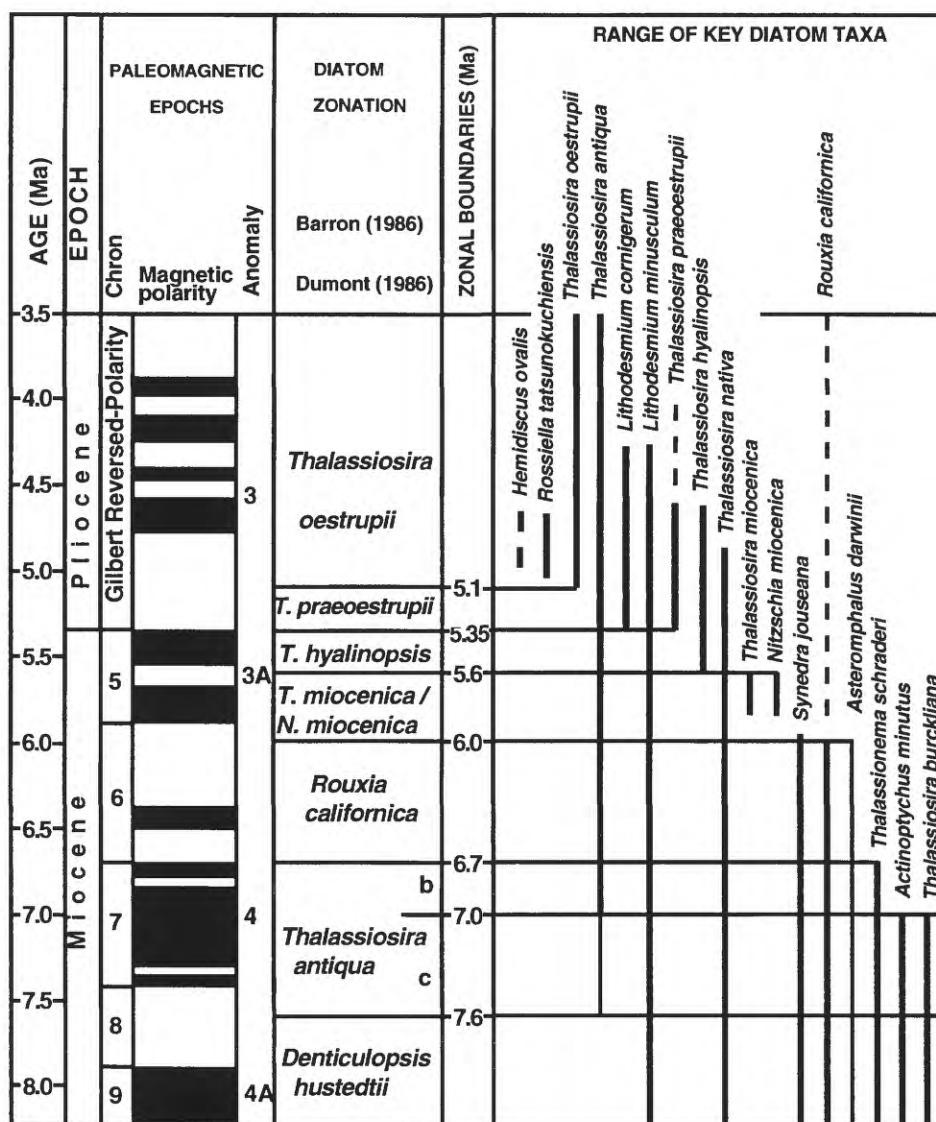
Figure 4. Diatom zones and species ranges used in this study. Also depicted are the key diatom taxa and their ranges. Slightly modified from Barron and Ramirez (1992).
