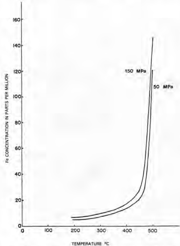
Figure 18. Isobars of Fe concentration in 1-m NaCl for the phases pyrite+pyrrhotite+gold+quartz in the system Fe-S-SiO_2-Au-NaCl-H_2O . From Rytuba (1977).
