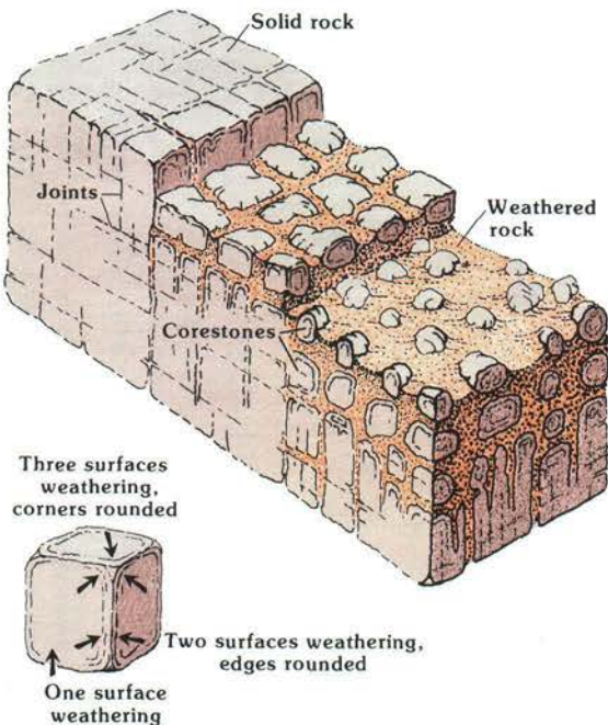
WEATHERING OF JOINT BLOCKS and stages in the formation of corestones. Corners and edges of granite blocks are attacked more readily by weathering along joints, and rounded corestones result. (Fig. 43)
