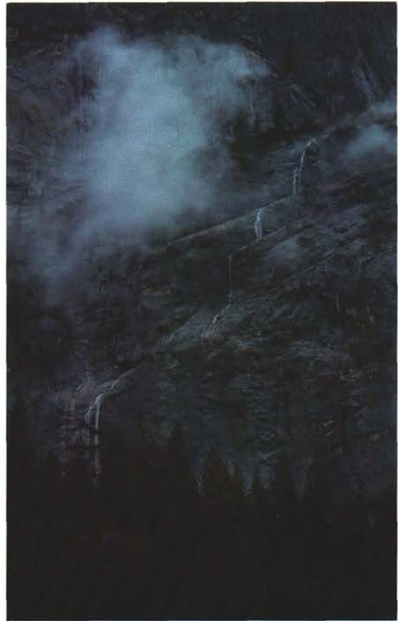
STAIRCASE FALLS. Stairtreads follow joints inclined eastward. Photograph by Tau Rho Alpha. (Fig. 35)
