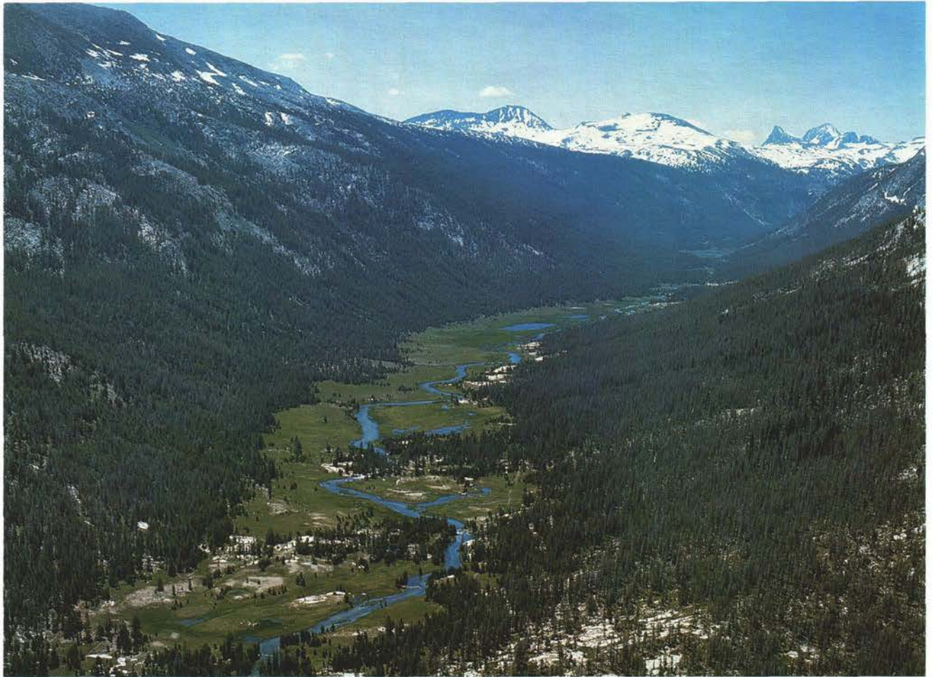
U-SHAPED GLACIATED VALLEY, the Lyell Fork of the Tuolumne River, looking southward. Photograph by Robert W. Cameron. © Cameron and Company; used with permission. (Fig. 68)
