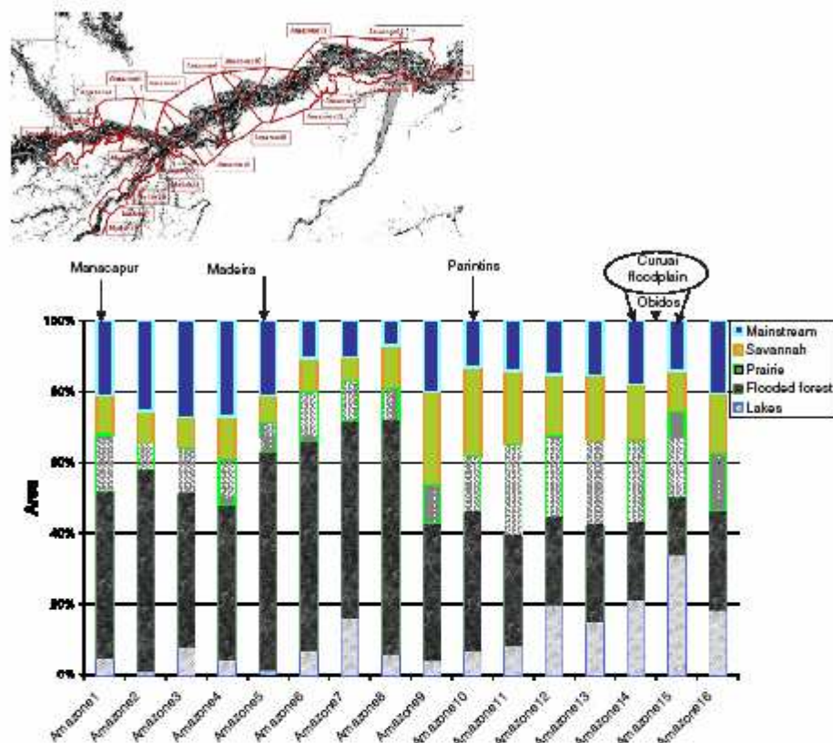
Figure 12 Distribution of wetland inundation and vegetation areas (in % of total \text{km}^2 per reach) for the 650 km reach of the Amazon River, between Manacapuru (on the Solimões R., downstream) and Santarém. Wetland extent and vegetation classes were mapped using mosaicked L-band synthetic aperture radar (SAR) imagery acquired by the Japanese Earth Resources Satellite-1, during low- and high-water periods. The five possible cover-state classes consisted of three vegetation cover classes, flooded forest, savannah and prairies, and two water permanent cover, flood plain lakes and mainstream River.
