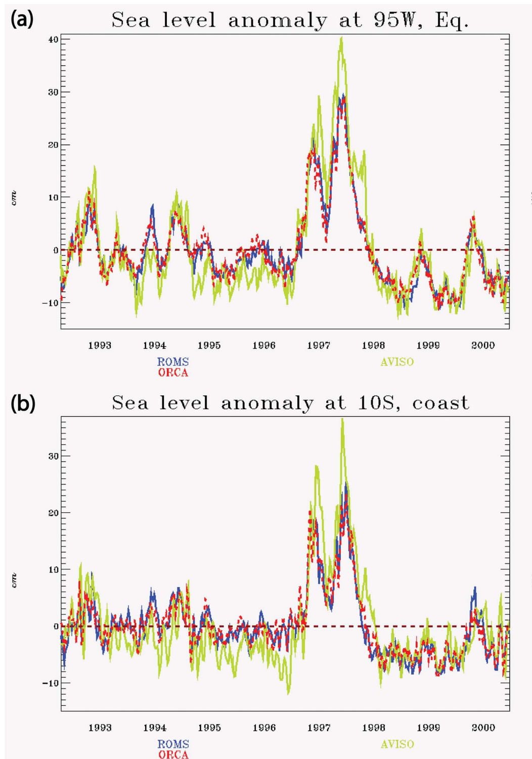
Figure 4. SLA (cm) simulated in R5d (solid blue line), in ORCA (dashed red line), and from AVISO data (solid green line) at (a) 0^{\circ}\text{N} , 95^{\circ}\text{W} and (b) 10^{\circ}\text{S} , 78.3^{\circ}\text{W} as a function of time. Units are cm.
