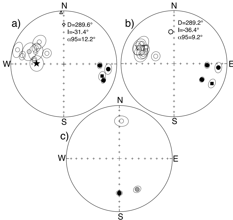
Figure 9. Equal-area stereonet of ChRM directions in (a) in situ and (b) after bedding correction for sites north of Chalhuanca. Circles are results in red beds and baked contacts, squares correspond to the antipodal magnetizations in limestones at site 72, and the star corresponds to the nonremagnetized limestone at site 71. The triangle, diamond, and hexagon are the present-day field direction, the geocentric axial dipole direction, and the expected direction at 40 Ma, respectively, from the Besse and Courtillot [2002] APWP for the South American plate. (c) Results in intrusive stocks 27 and 73 and remagnetized Jurassic black shales at site 34 (gray square).
