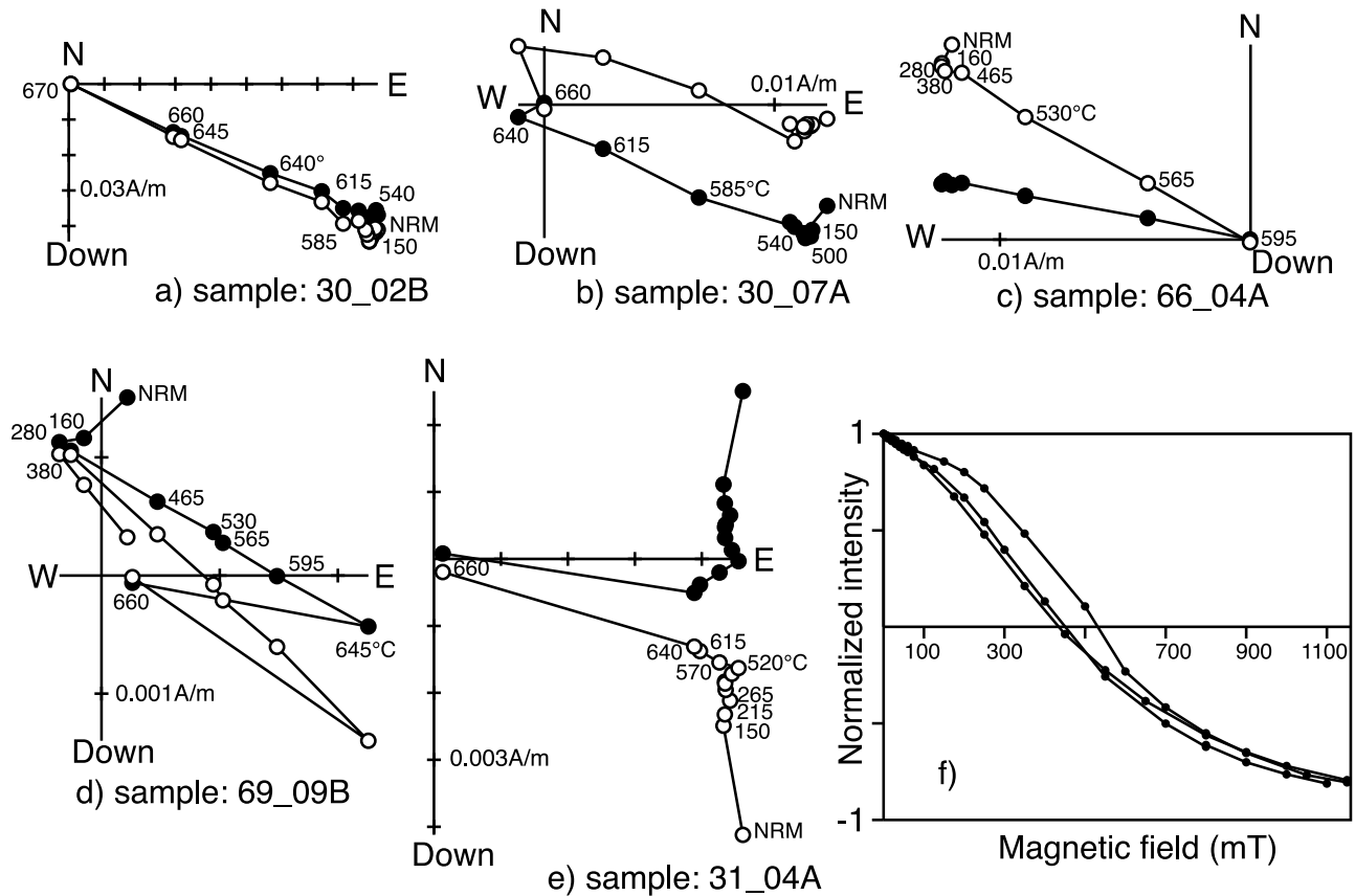
Figure 7. (a–e) Orthogonal plots of thermal demagnetization of samples from Paleogene red beds of the Chalhuanca area. Open circles are projection in the vertical plane, while circles correspond to the horizontal plane. (f) Back field IRM acquisition after saturation in a field of 2.5 T for red bed samples.
