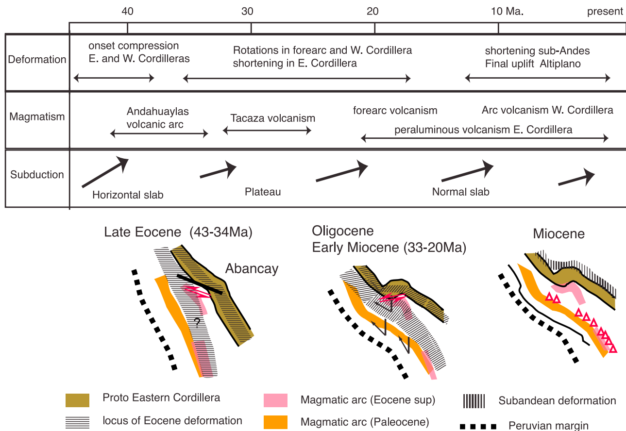
Figure 15. Summary of the geodynamic evolution of the southern Peruvian Andes since the middle Eocene. The Abancay line limits domains of central and southern Peru with different paleogeographic evolution [Carlotto et al. , 2009] and the protodeflexion was enhanced during Tertiary Andean deformation. A flat slab episode was proposed by James and Sacks [1999].
