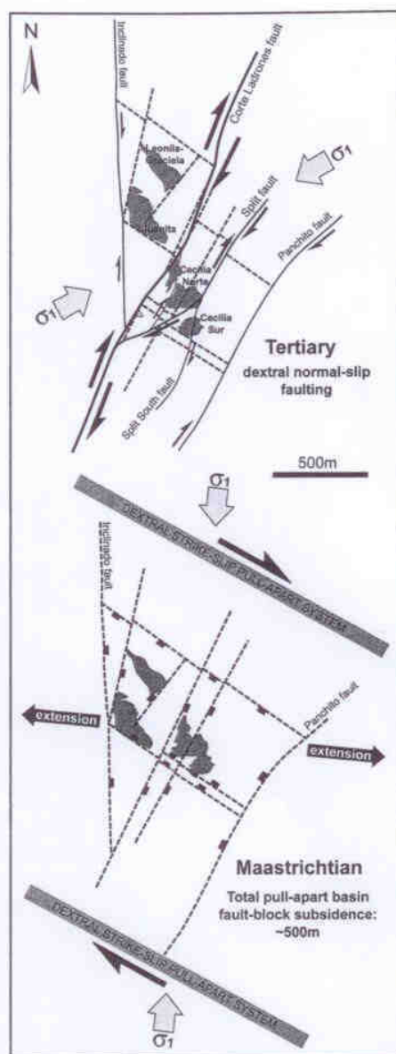
Fig. 5 Model for Late Cretaceous pull-apart origin of the Perubar basin. The tectonic stress ( \sigma_1 ) is inferred from relative plate motion reconstructions between the South American continent and the oceanic Farallon plate (e.g., Gordon and Jurdy 1986; Duncan and Hargraves 1984).
