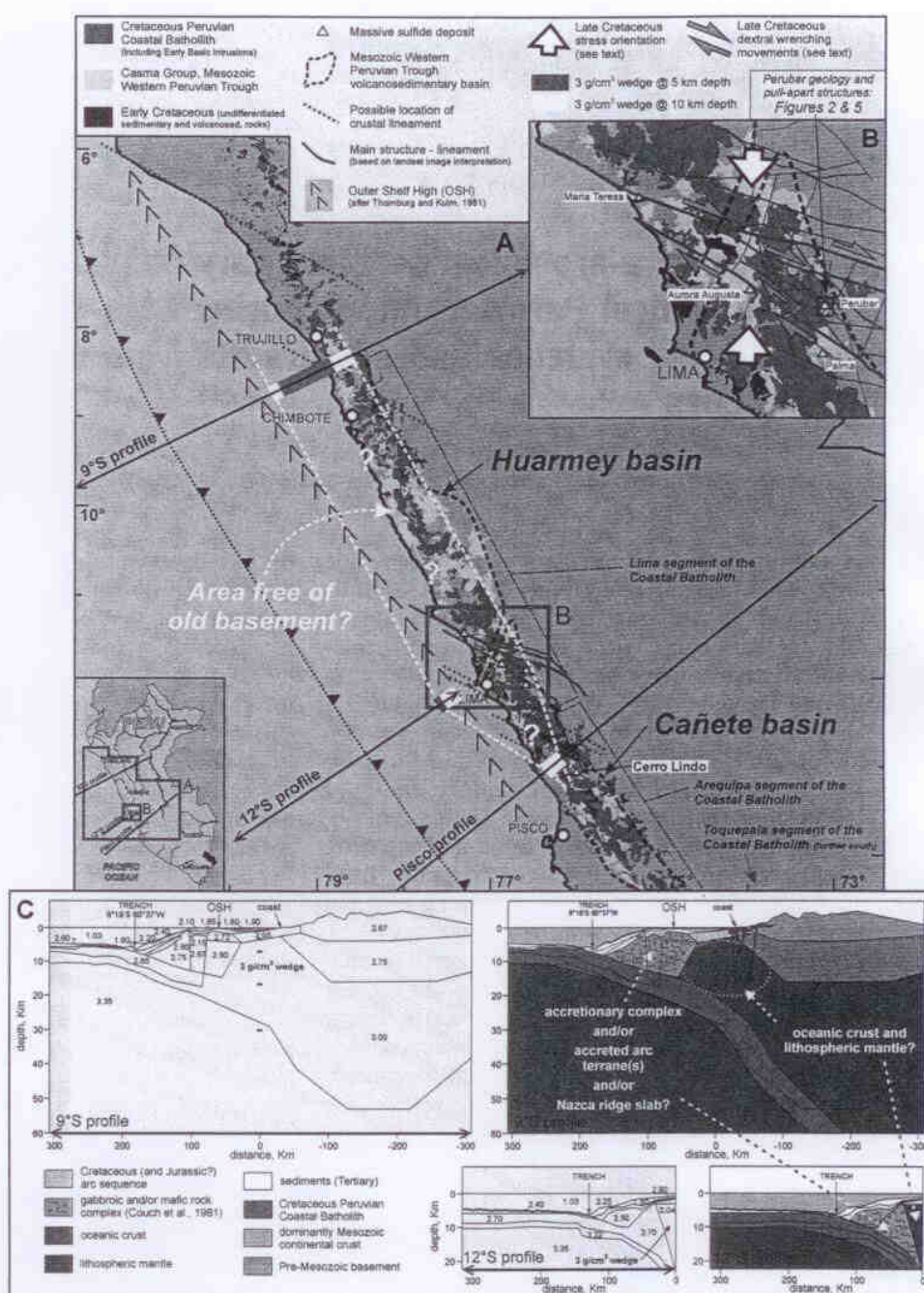
Fig. 1 a Geologic map of the Peruvian Coastal Batholith and Mesozoic Western Peruvian Trough (WPT) with related volcanosedimentary basins hosting massive sulfide deposits. Volcanosedimentary basin limits after Vidal (1987), Atherton et al. (1983), and Cobbing (1978). The yellow dotted lines encompass the 3.0 \text{ g/cm}^3 wedge at 10-km depth. Distribution of the Cretaceous Peruvian Coastal Batholith, Casma Group, and Early Cretaceous strata after the digital version of the geological map of Peru (INGEMMET 2000). b Main lineaments and structures based on Landsat-5 TM image (Red Band 7; Green Band 4; Blue Band 2) interpretation, downloaded from http://www.zulu.ssc.nasa.gov/mrsid/ . c Geologic interpretation of the deep structures along the 9°S and 12°S gravimetric, crustal and subcrustal cross sections (Couch et al. 1981; Jones 1981) of the continental margin of Peru
