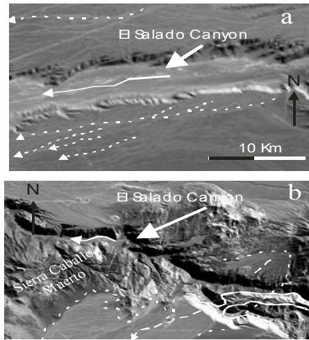
Figure 3: Morphologic features : a) E-W streams of the glacia surface in the Central Depression; b) Oblique Alluvial cone cuts by the EI Saldo canyon.
