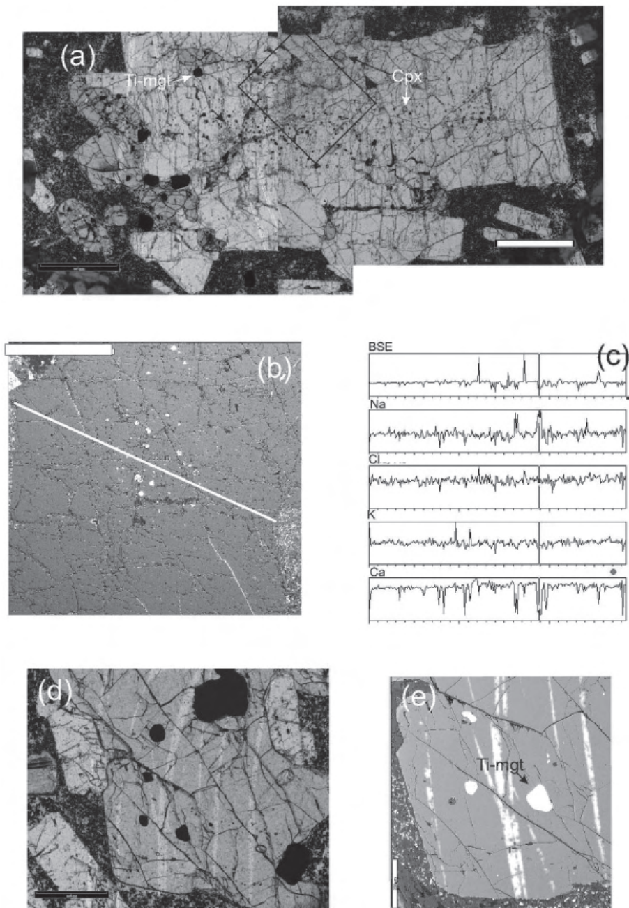
FIG. 5. a. Image of plagioclase from sample TC99-5a obtained with a polarised microscope (parallel light) showing small ( <10 \mu ) clinopyroxene (Cpx), Ti-magnetite (Ti-mgt) and fluid and melt inclusions. Scale bar: 0.5 mm; b. Scanning electron micrograph (back-scattered electron image) of a selected area of plagioclase phenocryst (see box in a) on which EDX compositional profiles were carried out; c. back-scattered topography (BSE) and Na, Cl, K and Ca EDX profiles (total profile length of 2853 \mu , see b) showing a rather chemical homogeneity; stronger Na and lower Ca variations coincide with small fractures as shown by vertical line in all spectres; d. Image of clinopyroxene from sample TC99-5a obtained with a polarised microscope (parallel light); e. Scanning electron micrograph (back-scattered electron image) of a selected area of a clinopyroxene phenocryst showing small subidiomorphic Ti-magnetite (Ti-mgt) inclusions; light lamellae are not related to differences in composition but with differences in C sputtering during manipulation of sample.
