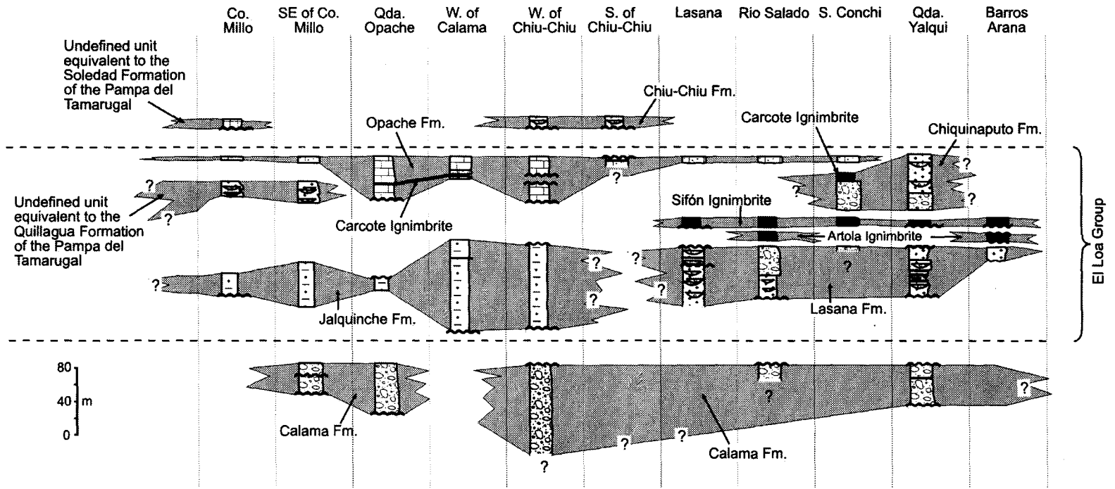
FIG. 4. Proposed lithostratigraphy for the Calama Basin. Lithologies and thicknesses correspond to those shown in figure 3. Six formations are recognised within the proposed stratigraphy. The Calama Formation comprises the basal unit of the basin-fill. It is overlain by the El Loa Group, which consists of the Jalquinche, Opache, Lasana, and Chiquinaputo formations. The uppermost strata comprise the Chiu-Chiu Formation. See text for discussion.
