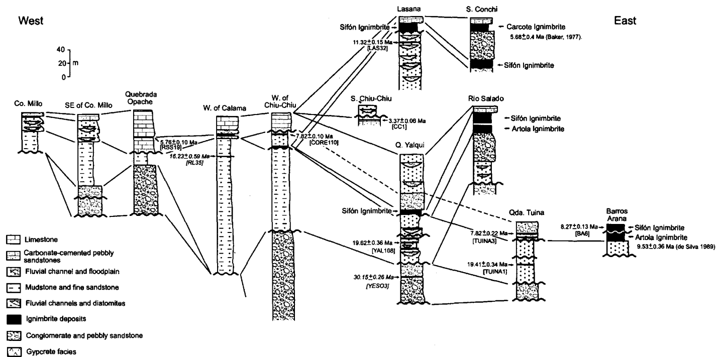
FIG. 3. West to east stratigraphy of the Calama Basin. See figure 2 for the location of sections studied. Correlations are based on the dated volcanic ashes and ignimbrites, unconformities and lithological similarities. Sample numbers for the volcanic ashes and ignimbrites are given in brackets and correspond to those presented in table 2. Age dates in italics are from reworked ashes.
