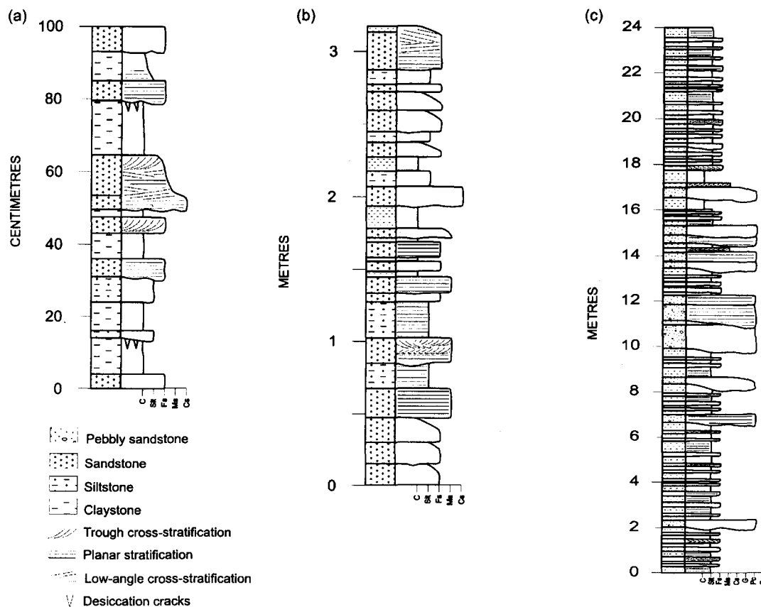
FIG. 7. Representative sedimentary logs through part of the Jalquinche Formation exposed in (a) the Río Loa valley 10 km east of the Cerro Millo high ( 22^{\circ}51'S/69^{\circ}19'W ); (b)- Río San Salvador valley at the Cerro Millo high ( 22^{\circ}50'S/69^{\circ}24'W ) and (c) the Río Loa gorge, 10 km west of Calama ( 22^{\circ}31'S/69^{\circ}01'W ).
