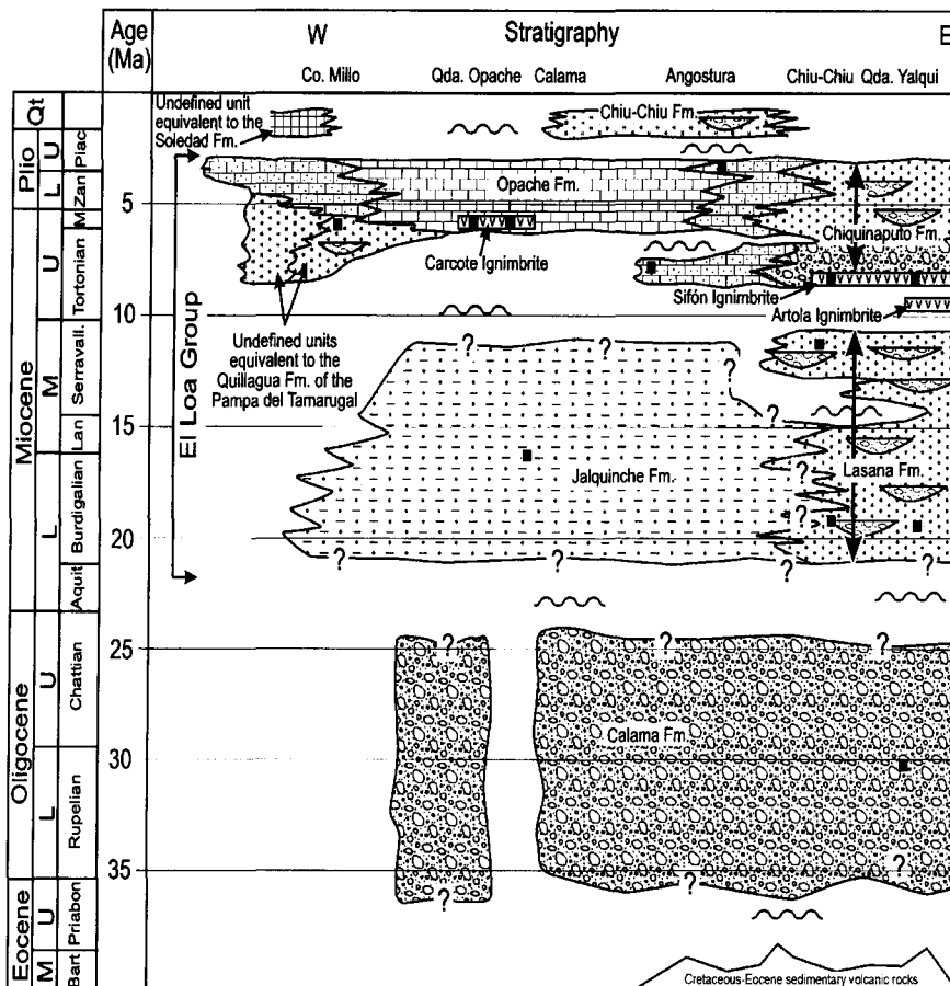
FIG. 5. Chronostratigraphic correlation of the Oligocene to Recent succession within the Calama Basin from Co. Millo in the west to Quebrada Yalqui in the east. The spatial and temporal development of angular unconformities are shown. Formation names correspond to proposed redefinition of the Calama Basin stratigraphy (see text). The dated ashes described in the text are indicated by the ■ symbol. Bart-Bartonian; Priabon-Priabonian; Aquit-Aquitian; Lan-Langhian; Serravall-Serravallian; M-Messinian; Zan-Zanclian; Piac-Piacenzian. Cretaceous-Eocene sedimentary volcanic rocks-Cretaceous to Eocene sedimentary and volcanic strata.
