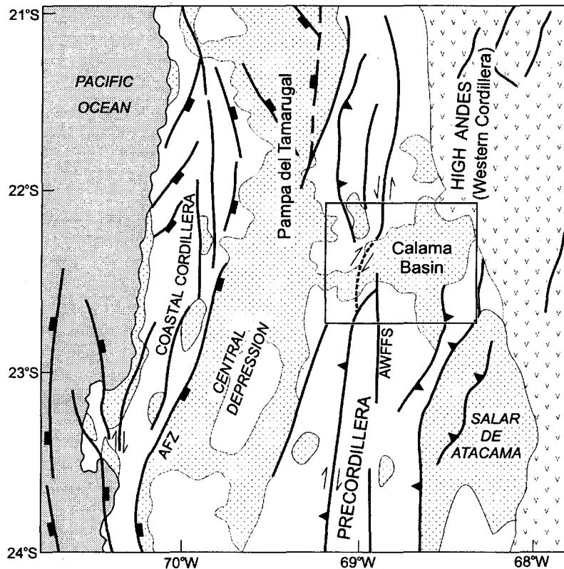
FIG. 1. General distribution of Tertiary (post-Eocene) sedimentary basins in the north Chilean forearc. Box outlines area of figure 2. AFZ = Atacama Fault Zone; AWFFS = Argomedo-West Fissure Fault System. Stipple pattern indicates late Eocene to Holocene basins; v= volcanic arc, unpatterned area is pre-Eocene basement.
