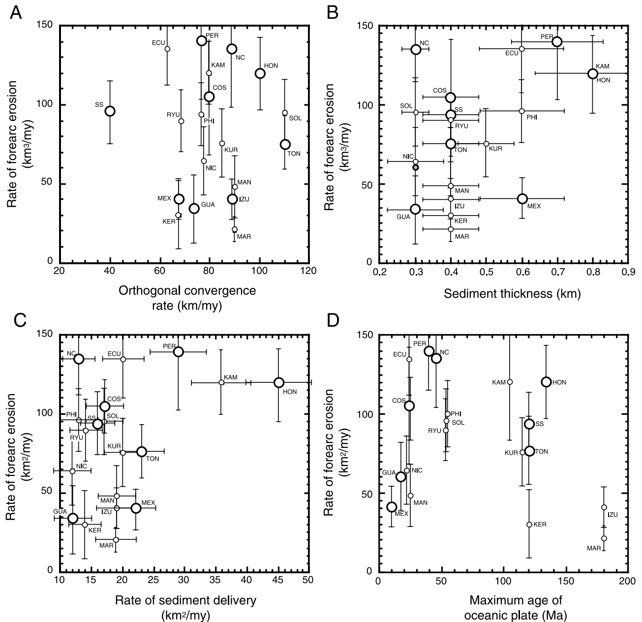
Figure 11. Diagrams showing the interrelationships between the rate of forearc erosion and a variety of tectonic criteria that were significant in controlling the rate of sediment off scraping in accretionary margin settings. In the case of erosive plate margins, no such simple control is recognized. Large circles show margins for which the rate of tectonic erosion has been quantified, while the small circles show margins for which a tectonic erosion rate is inferred by comparison.
