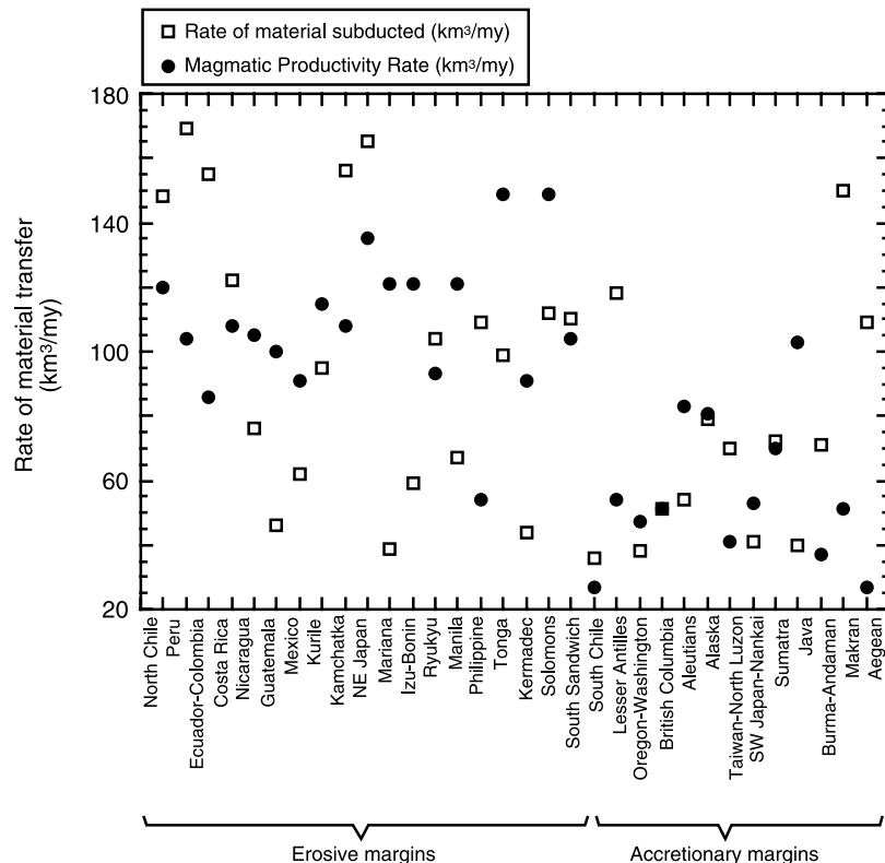
Figure 18. Diagram showing the relative rates of material subduction compared to magmatic productivity in the world's major subduction zones. The arcs of the erosive margins could theoretically be sourced from the recycling of subducted materials, while the accretionary margins require new extraction of crust from the upper mantle.
