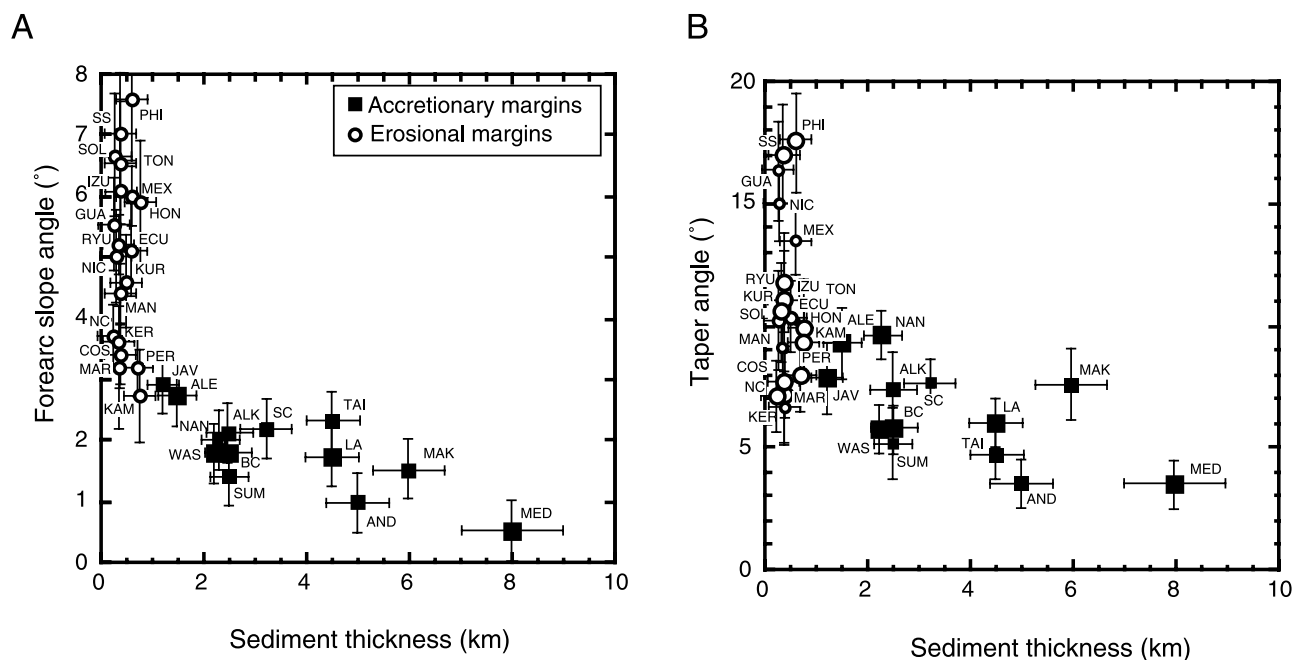
Figure 8. Diagram showing the inverse relationship between the thickness of sediment at the trench on the subducting plate and (a) the long wavelength slope of the forearc and (b) the taper of the forearc wedge.
