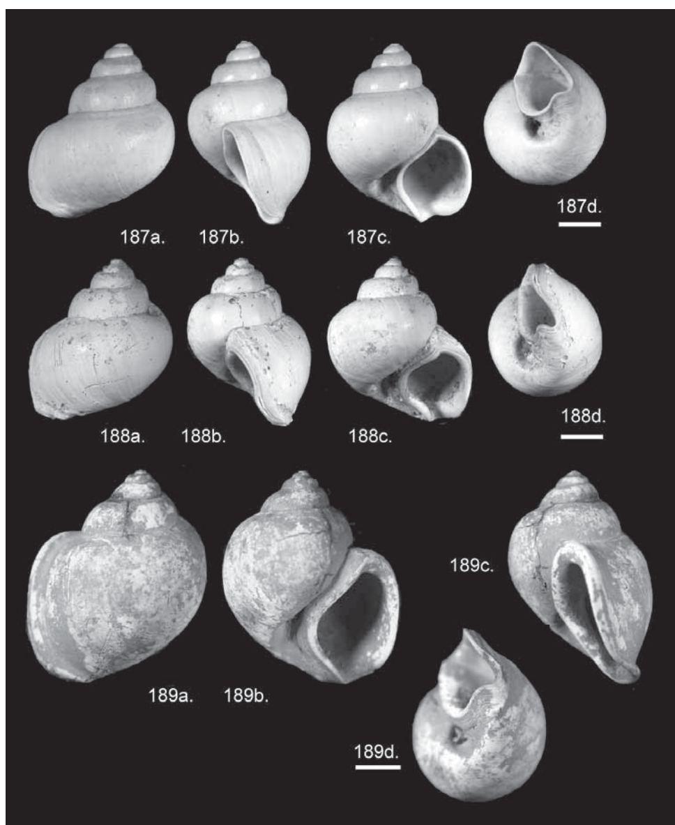
Fig. 187. Sioliella crassilabra (Conrad, 1871). RGM 456 324, San Miguel de Cochiquinas (Loreto, Peru). a, rear view. b, lateral view. c, front view. d, basal view.
