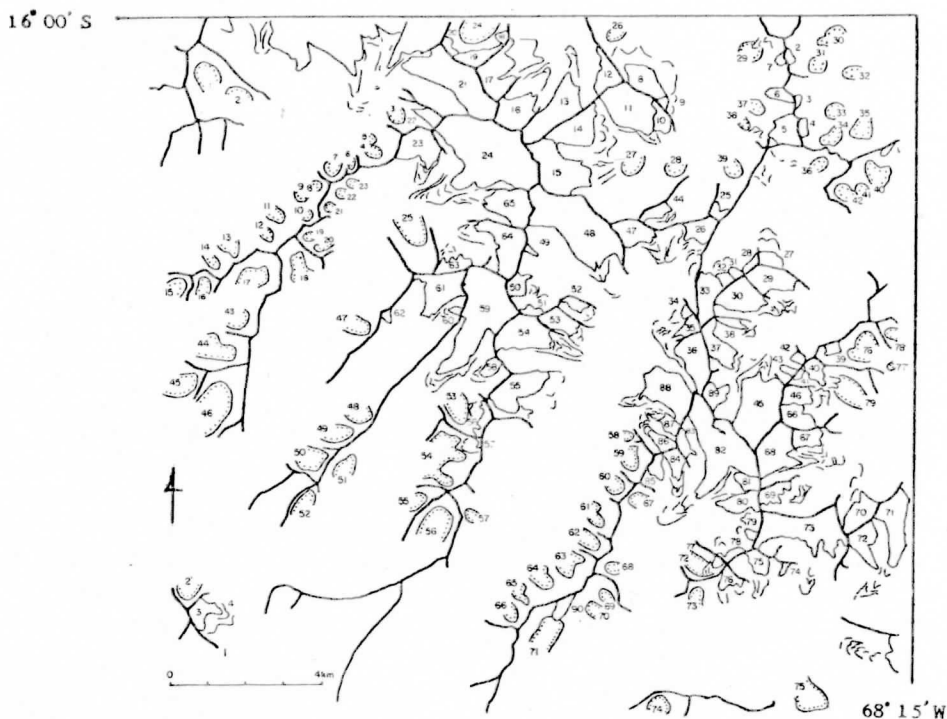
Fig. 1 Distribution of glaciers and cirques in the quadrangle "Lago Khara Kkota", Bolivia (after Nogami, 1968)
