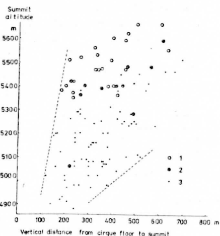
Fig. 3 Summit altitude vs. vertical distance from cirque floor to summit
