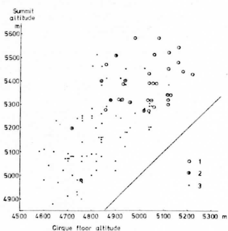
Fig. 2 Summit altitude vs. cirque floor altitude
