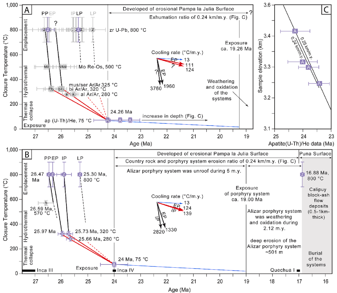
Fig. 4. Summary diagram of integrated zircon U-Pb, biotite-alunitite ^{40}\text{Ar}/^{39}\text{Ar} , and apatite (U-Th)/He data from La Arena and Alizar, are also plotted here U-Pb, Re-Os, and ^{40}\text{Ar}/^{39}\text{Ar} data (gray symbols) reported by Montgomery (2012) and Santos (2020) , which records a complete cooling history of the La Arena-Calaorco (A) and Alizar-Vanessa (B) porphyry-epithermal systems. All age determinations are shown with 2\sigma uncertainty. Results of geochronological data reveal multiple cooling path with rapid to moderate cooling rates ( ^{\circ}\text{C}/\text{m.y.} ) as a result of each of the porphyry intrusions (PP: precursor pluton, EP: early porphyry, IP: inter-mineral porphyry, and LP: late-mineral porphyry). The protracted cooling history at La Arena and Alizar lasted \sim 7.46 and \sim 7.12 m.y., from emplacement and associated hydrothermal activity in 0.25 and 0.36 m.y. (black lines, dashed where uncertain), through thermal collapse in 2.21 and 1.76 m.y. (red lines, dashed where uncertain), to common exposure interval of 5 m.y. (blue lines), respectively. Weathering and oxidized during 2.12 m.y. led to deep erosion ( \sim 500 m thick) at Alizar, comparable with preserved leach capping ( \sim 400 m thick) at adjacent La Arena. Subsequent volcanic activity at ca. 16.88 \pm 0.05 Ma, leading to burial of the deposits and partially preservation of the telescoped porphyry-epithermal systems. C. Age-elevation diagram for apatite (U-Th)/He dating results ( 2\sigma ) from La Arena and Alizar. Data ages plot on a well-defined younging trend with increasing depth, error-weighted slope of 0.24 and 0.25 km/m.y., consistent with 0.24 km of rapid exhumation at \sim 24 Ma best fits existing data. (For interpretation of the references to colour in this figure legend, the reader is referred to the web version of this article.)
