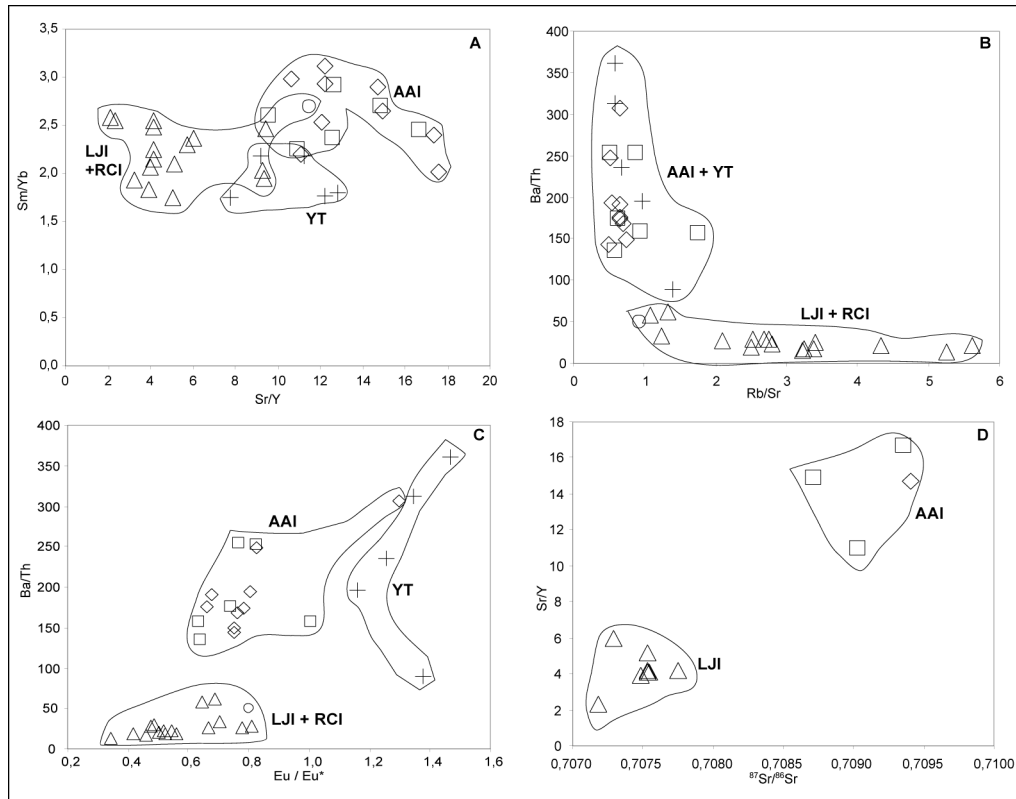
Figure 2 : Trace elements, trace elements ratio and Sr isotopes discriminant plots for Arequipa area ignimbrites. A) Sm/Yb versus Sr/Y (indicators of depth of assimilation, garnet signature), B) Ba/Th v. Rb/Sr, C) Ba/Th v. Eu/Eu*, and D). Sr isotopic composition versus Sr/Y.
