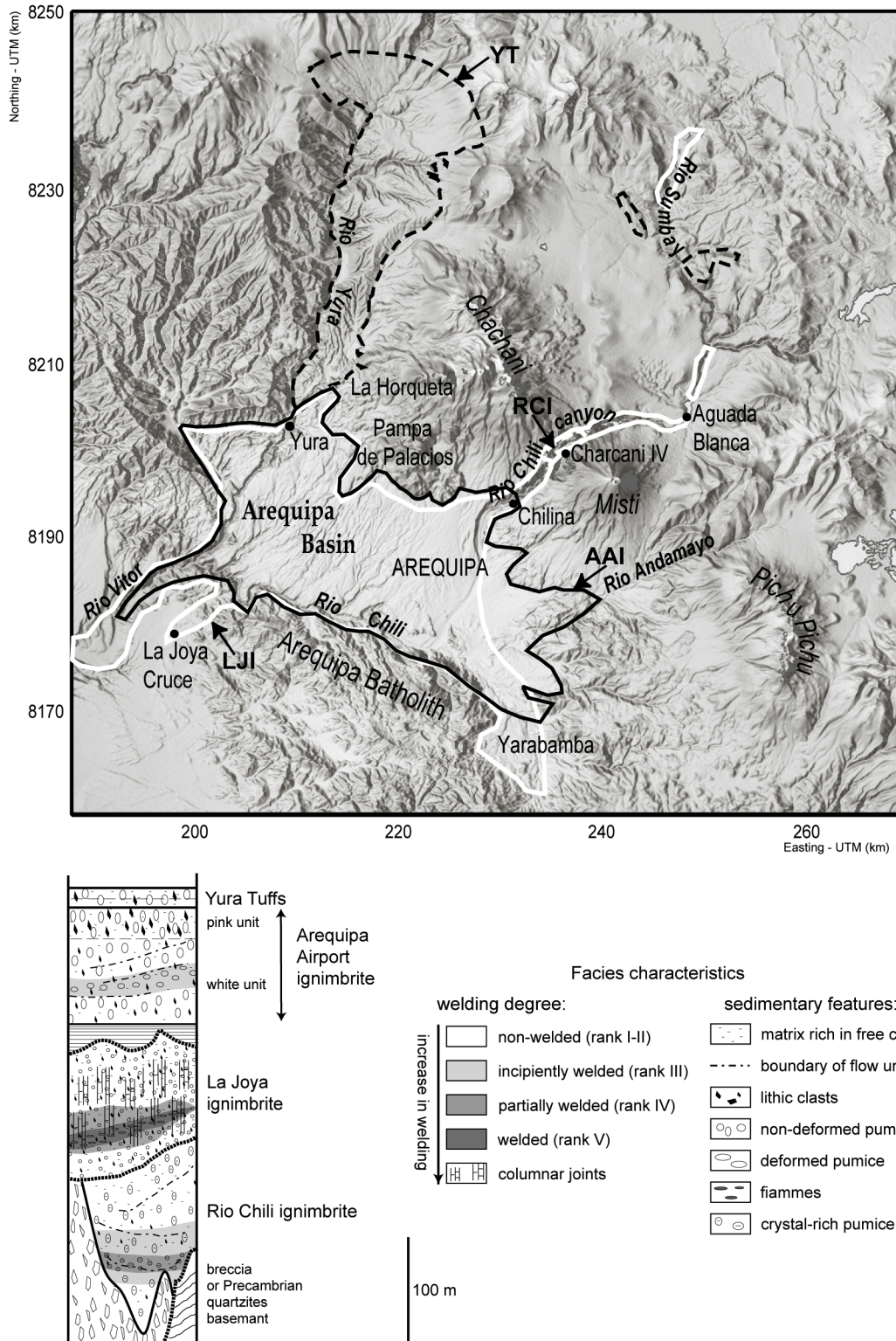
Figure 1 : DEM of the Arequipa area (from the USGS web site), showing locations quoted in the text. The approximate boundaries of the four ignimbrites are shown. Synthetic stratigraphic section of the Neogene ignimbrites of the area of Arequipa with facies characteristics.
