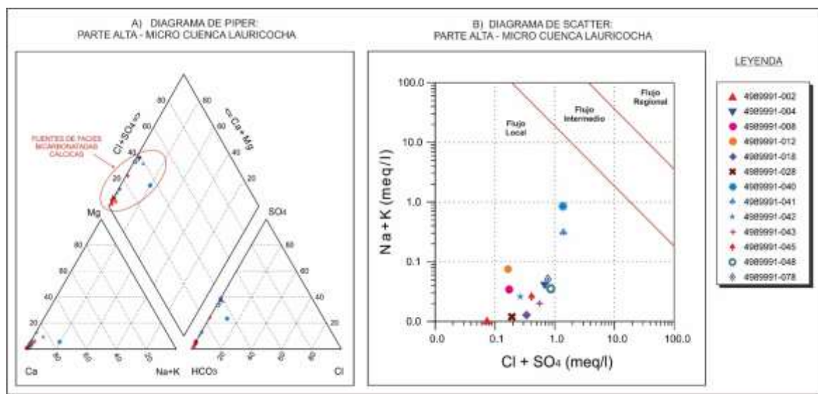
Figure 4: Scatter and Piper diagram for groundwater sources located on the top of the Lauricocha Subcatchment.
