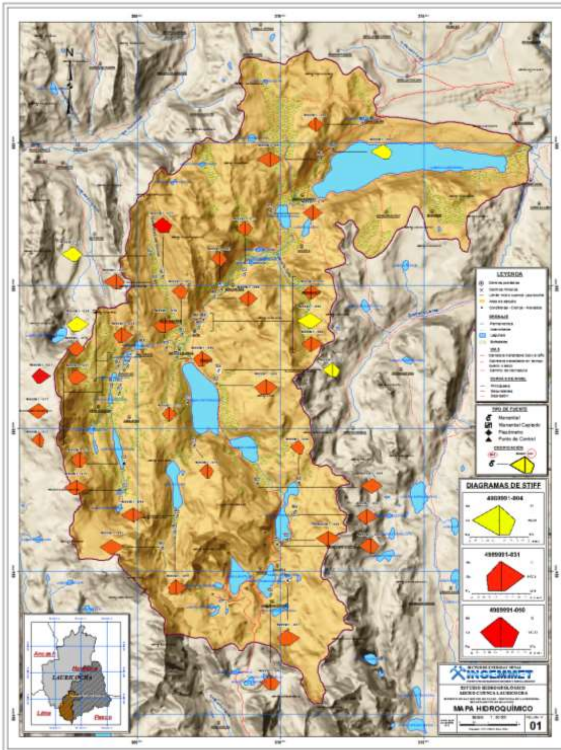
Figure 3: Hydrochemical map Lauricocha watershed.
