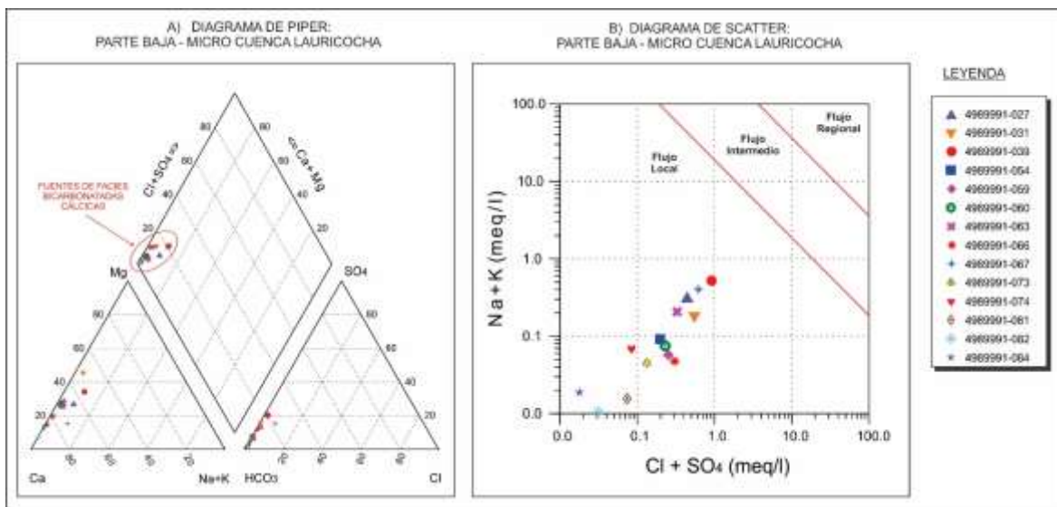
Figure 6: Piper and Scatter diagram for groundwater sources located in the lower part of the Lauricocha Sub catchment.
