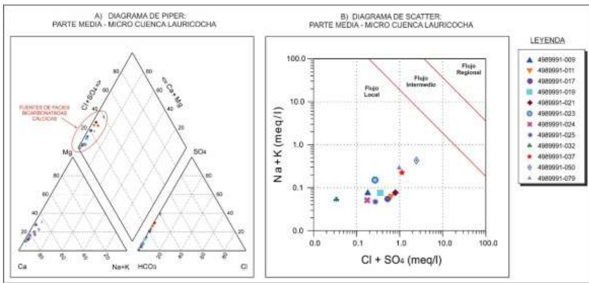
Figure 5: Piper and Scatter diagram for groundwater sources located in the middle of the Lauricocha Subcatchment.
