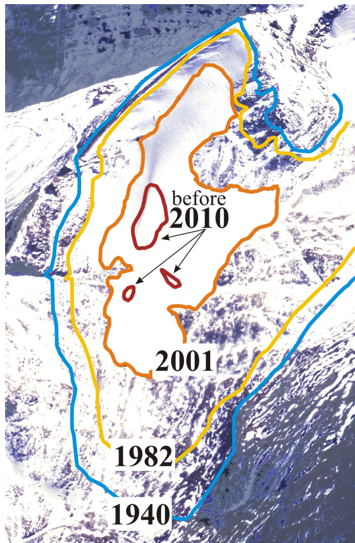
Fig. 1 Shrinkage of the Chacaltaya Glacier in Bolivia (16°S): observations and projections. Highest altitude of the glacier in 1940: 5395 m a.s.l.; surface area of the glacier in 1940: 0.223 km 2 , in 2001: 0.048 km 2 . (Photo, dated 2001, and estimates of the glacier extent are by Bernard Francou). Now (2005), Chacaltaya is already divided into three parts and the whole glacier may disappear before 2010.
