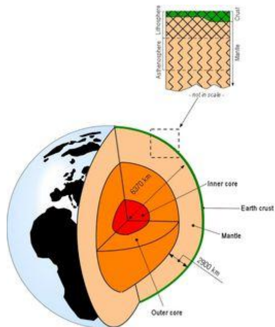
Figure 1: The Earth's crust, mantle, and core. Top right: a section through the crust and the uppermost mantle.
