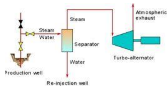
Figure 11: Sketch of an atmospheric exhaust geothermal power-plant. The flow of geothermal fluid is indicated in red.
