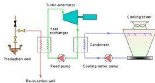
Figure 13: Sketch of a geothermal binary power plant. The flow of geothermal fluid is in red, the secondary fluid in green, and the cooling water in blue.
