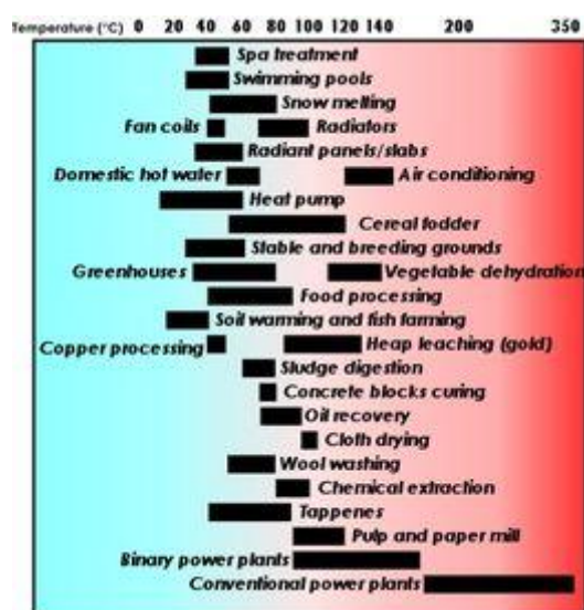
Figure 10: Diagram showing the utilization of geothermal fluids (derived from Lindal, 1973)
