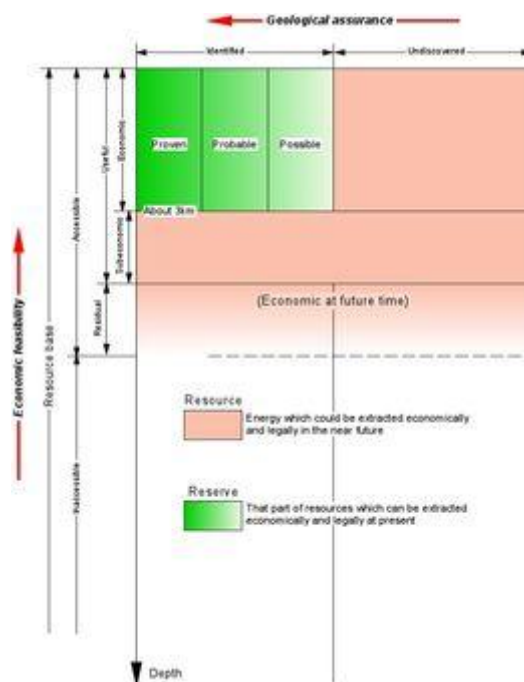
Figure 9: Diagram showing the different categories of geothermal resources. (From Muffler and Cataldi, 1978). The vertical axis is the degree of economic feasibility; the horizontal axis is the degree of geological assurance.
