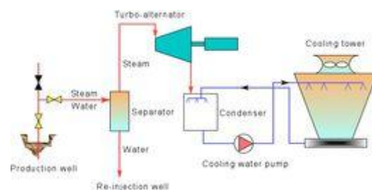
Figure 12: Sketch of a condensing geothermal power-plant. The flow of high-temperature fluid is indicated in red, and the cooling water in blue.
