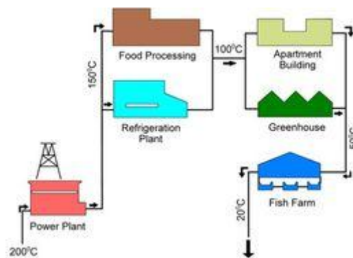
Figure 20: Cascade uses of geothermal energy (courtesy of the Geo-Heat Center, Klamath Falls, Oregon, USA)
