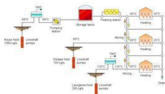
Figure 14: Simplified flow diagram of the geothermal district heating system of Reykjavik. (From Gudmundsson, 1988)
