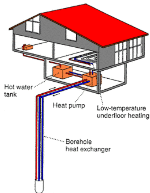
Figure 15: Typical application of ground-coupled heat pump system (from Sanner et al., 2003).
