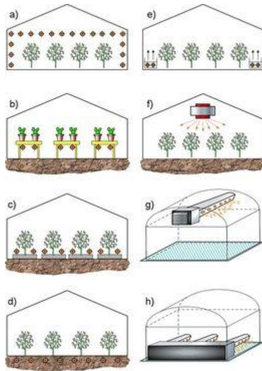
Figure 18: Heating systems in geothermal greenhouses. Heating installations with natural air movement ((natural convection): (a) aerial pipe heating; (b) bench heating; (c) low-position heating pipes for aerial heating. (d) Soil heating. Heating installations with forced air movement (forced convection): (e) lateral position;(f) aerial fan; (g) high-position ducts; (h) low-position ducts. (From von Zabeltitz, 1986.)
