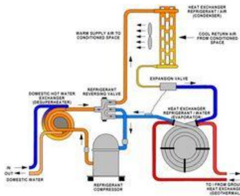
Figure 16: Sketch of a heat pump in heating mode (courtesy of the Geo-Heat Center, Klamath Falls, Oregon, USA)
