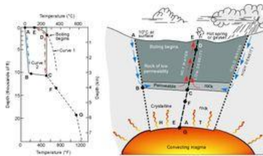
Figure 7: Model of a geothermal system. Curve 1 is the reference curve for the boiling point of pure water. Curve 2 shows the temperature profile along a typical circulation route from recharge at point A to discharge at point E (From White, 1973).
