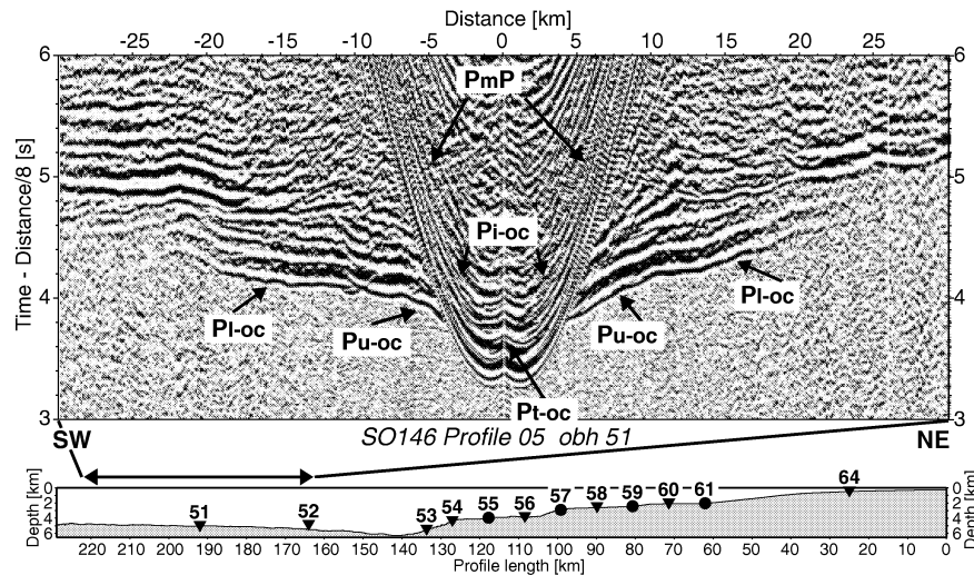
Figure 6. Near-offset traces of the wide-angle seismic section recorded by OBH 51 located on the oceanic crust on profile SO146-5/12°S. The data are displayed with a reduction velocity of 8 km s -1 . P_{t-oc} , P_{i-oc} and P_mP are reflections from the top of the oceanic crust, the intracrustal boundary and the crust–mantle boundary. P_{u-oc} and P_{l-oc} are refractions from the upper oceanic crust and the lower oceanic crust. The topography along the entire profile is shown underneath the seismic section with all the locations of the OBH/S stations; triangles and circles mark OBH and OBS stations, respectively.
