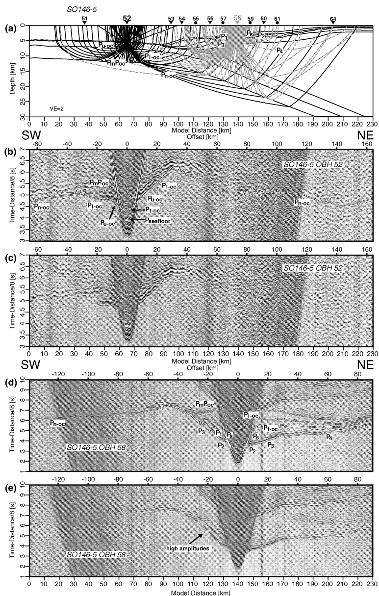
Figure 8. Record sections OBH 52 (a, b and c) and OBH 58 (a, d and e) of profile SO146-5/12°S. See Fig. 7 for details and definitions of abbreviations. The seafloor reflection in record section OBH 52 is not coincident with the direct arrival, because the instrument was placed 600 m above the seafloor.
