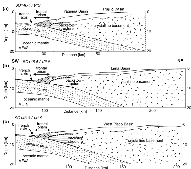
Figure 15. Structural models from north to the south. Line drawings at the toe of the margin are incorporated from earlier reflection seismic studies (Kulm et al. 1981; von Huene & Suess 1988). The structure of the backstop has been inferred from P -wave velocities derived from the refraction seismic data. The dotted area is characterized by lower seismic velocities than the landward part of the continental crust. The bold line at the continental/oceanic plate boundary marks the zone where we assume that basal erosion is most effective. The grey area for all three profiles contains the pixel information for the calculation of the frontal prism volumes.
