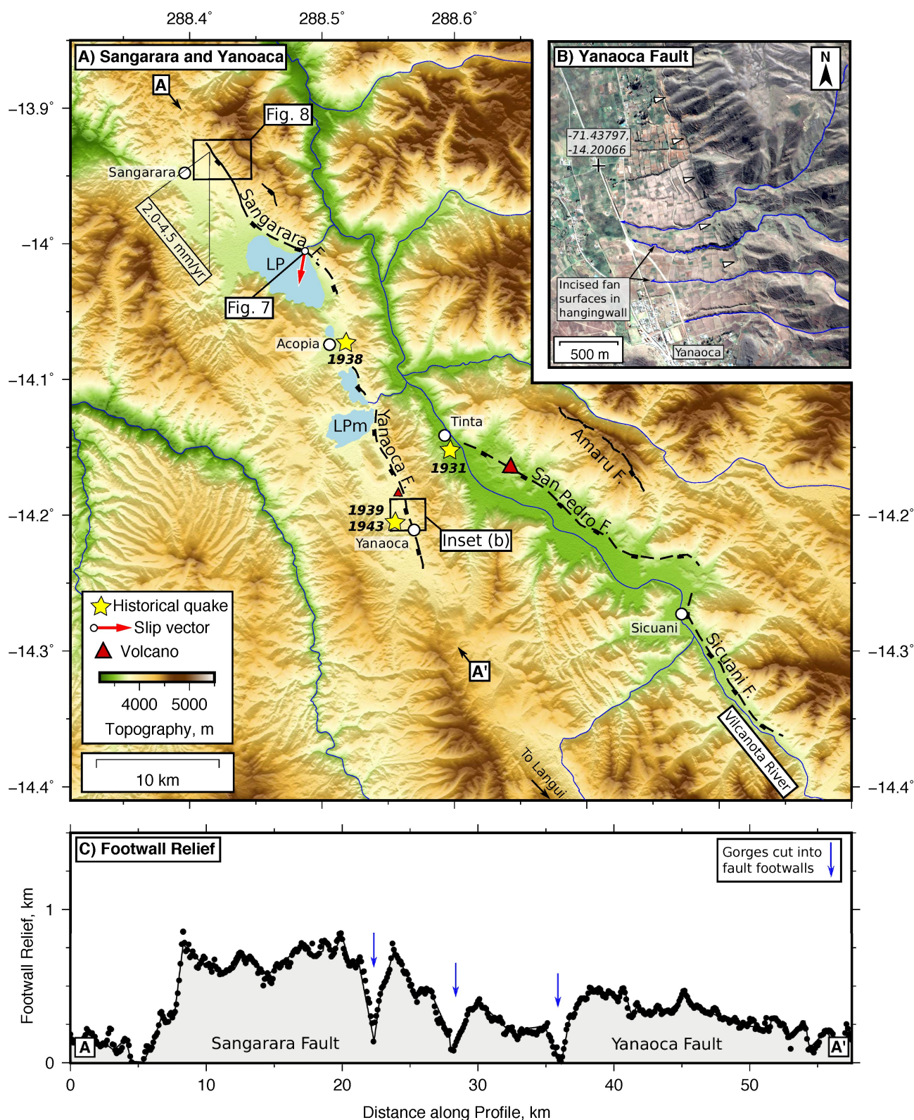
Figure 6: Overview of the active faulting between Sangarara and Yanoaca. (a) SRTM 30 m DEM overlay with active faults. The legend is the same as in Fig. 2. The two lakes are: LP = Lake Pomacanchi and LPm = Lake Pampamarca. (b) Digital Globe imagery from Google Earth of incision across the bedrock-alluvium contact along the Yanoaca Fault. Incision is also present in the hangingwall fan surfaces at Sangarara (see Fig. 8). (c) Footwall relief along the Sangarara-Yanoaca valley.
