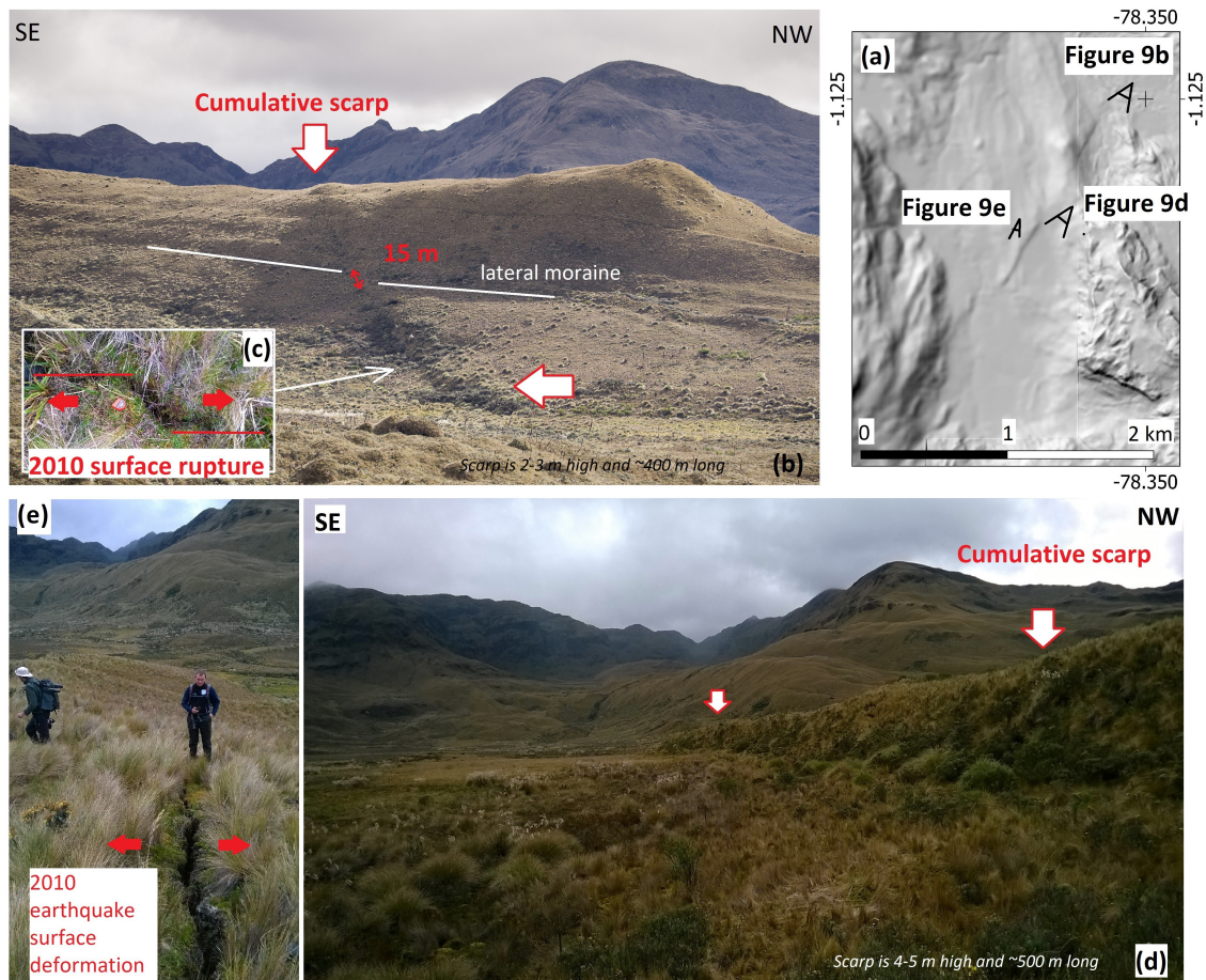
FIGURE 9 | (a) The Pisayambo Fault segment has ruptured during a small magnitude event ( M_w \sim 5 ) in 2010 along a clear cumulative fault scarp, leaving a 9 km long surface rupture (Champenois et al., 2017). (b,c) In the central section of the rupture, view of the 15 m offset of a lateral moraine, with evidences of 2010 30–40 cm right-lateral surface rupture; (d) illustration shows a high cumulative scarp in the south-central section, with coseismic surface deformation (open fissure).
