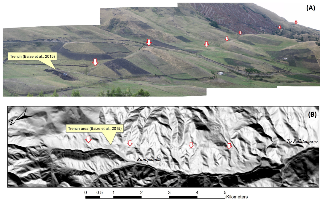
FIGURE 2 | Illustration of the signature of an active portion of the Pallatanga fault on a field panorama (A) and on the corresponding 4 m resolution DEM (B). On the left of the photo in (A), one can observe one of the trenches dug in 2009–2010 and presented in Baize et al. (2015). The fault trace is easily inferred from an uphill-facing and counter-slope scarp, matching a deflection in perpendicular morphological features (channel incisions, ridges). See Figure 3 and Supplementary Figure S8 for location.
