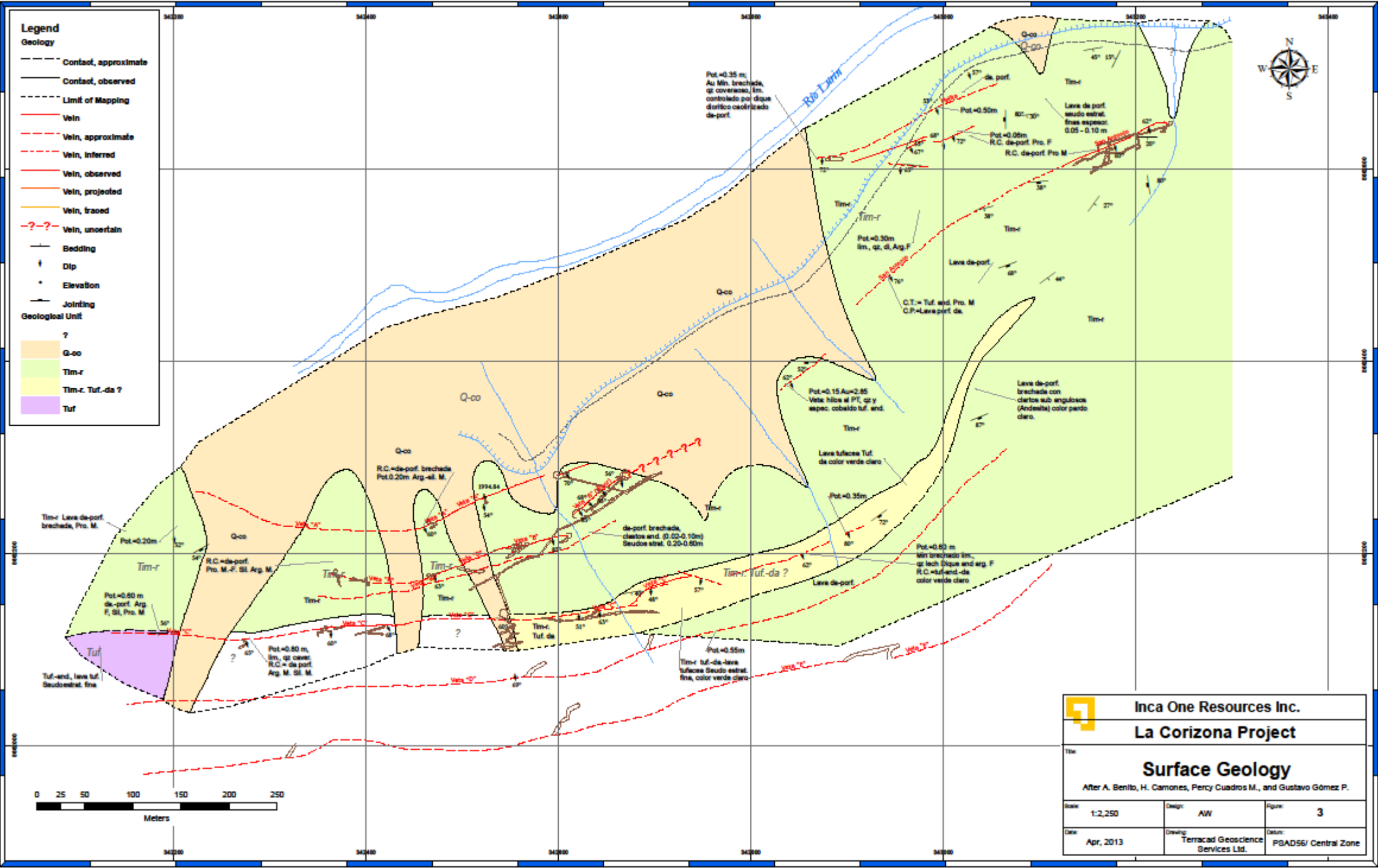
Figure 5 Surface Geology Map
