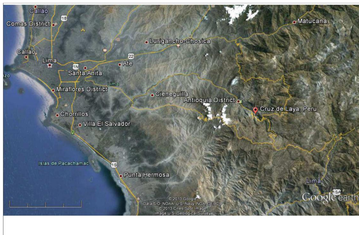
Figure 2 La Corizona Project is 85 km southeast of Lima near Cruz de Laya
