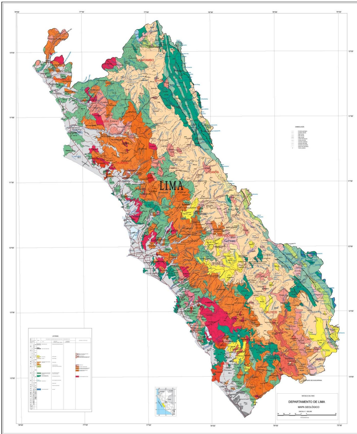
Figure 7 Geology of Lima Department
