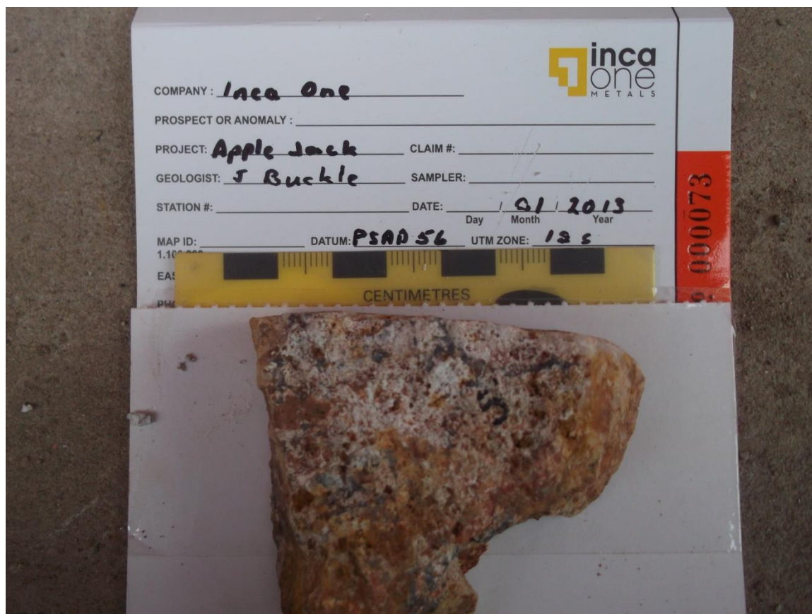
Figure 12 Hand sample 5 kaolinite-limonite-hematite-quartz hydrothermal alteration
