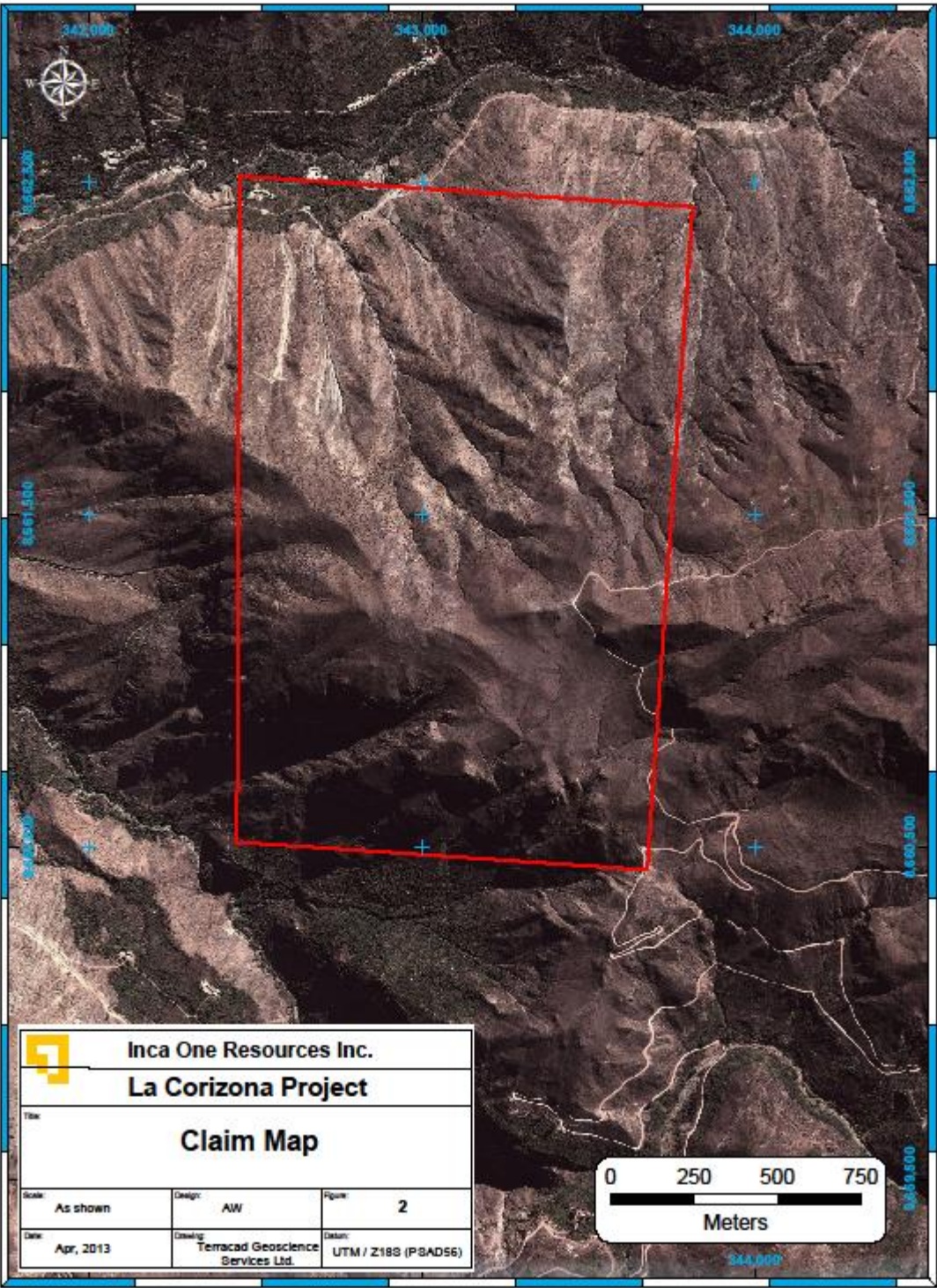
Figure 4 Location Satellite Image
