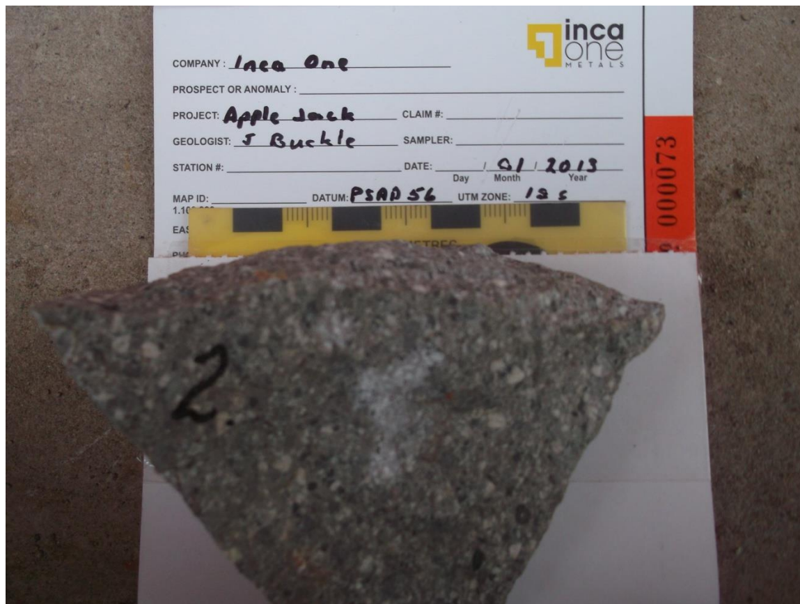
Figure 9 Hand sample 2 typical andesite-dacite medium grained tuff
