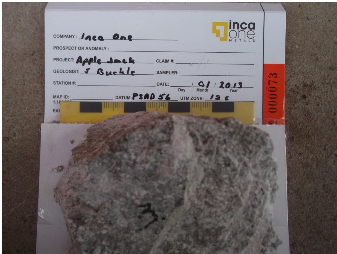
Figure 10 Hand sample 3 kaolin-argillite altered tuff and quartz veins with minor hematite and minor disseminated pyrite
