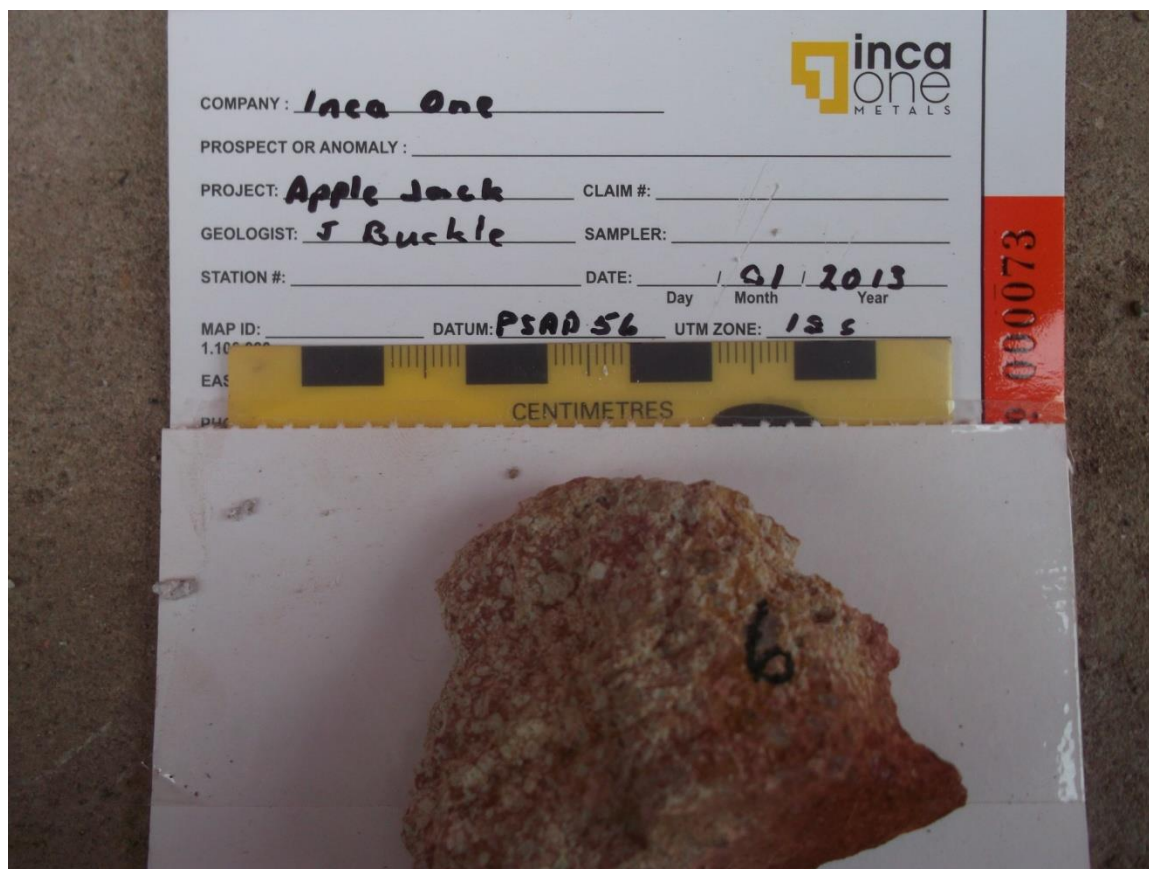
Figure 13 Hand sample 6 jarosite-limonite altered matrix in tuff
