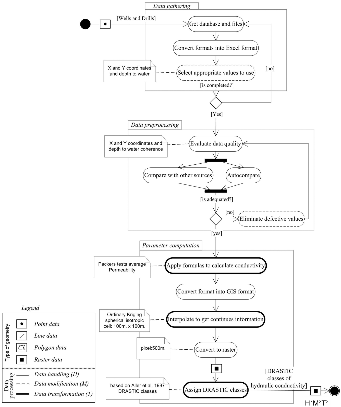
Fig. 2. Formalization of data processing required to estimate the DRASTIC parameter – HYDRAULIC CONDUCTIVITY.
