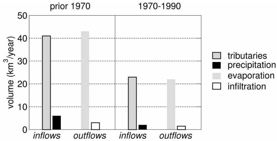
Fig. 5: (from up to low) Level variation of Lake Tchad from altimetry multi-mission (T/P (up to 2002), Envisat (up to 2008) and Jason-2(up to 2010)) (a), surface variations from Modis images (b) and water balance of the lake (c).
