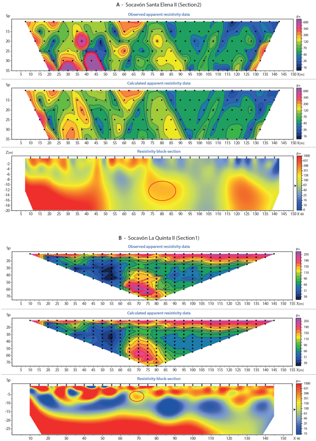
FIG. 7. A. Santa Elena Socavón. B. La Quinta Socavón. Upper panel: pseudosection of the observations. Middle panel: model response. Lower panel: 2D model inversion section (in red circle, the interpreted socavón in agreement with the conceptual model). The vertical scale in the pseudo sections is apparent depth and the coloured resistivities are apparent resistivities (an integral of the resistivity between the current injection point and the voltage measured point). Observation and model response should match if the model is correct. The inversion section depth is in meter and resistivity corresponds to the resistivity distribution in the space.
