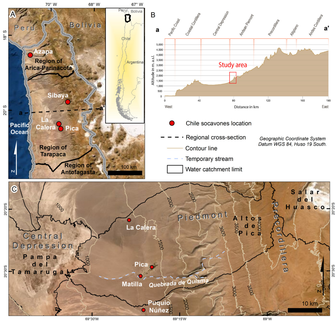
FIG. 2. Location of the study area. A. Location of Chile socavones; B. Topographic and geomorphological profile W-E of Chile at the latitude of the study area; C. Map of Pica area.
